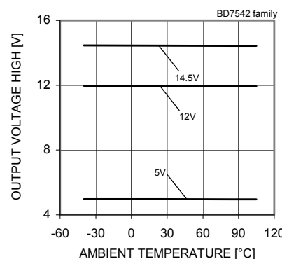
Fig. 75 Output Voltage High - Ambient Temperature (RL=10[kΩ])
