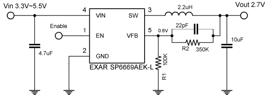
Fig. 18: Adjustable Output Voltage Version Typical Application Circuit
