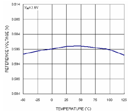
Fig. 7: Reference Voltage vs Temperature
