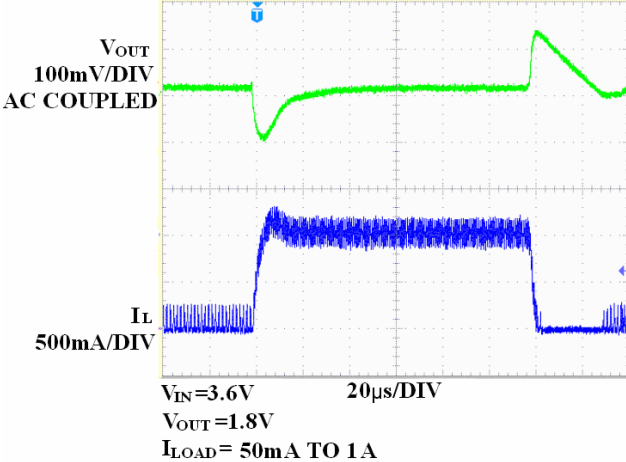
Load Step
