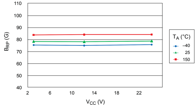
Release Point versus Average Supply Voltage
