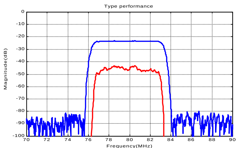
LBN80-6.8 SAW Filter Typical Performance
