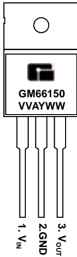
TO 220
