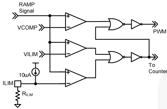
Figure 33. ILIM Network
