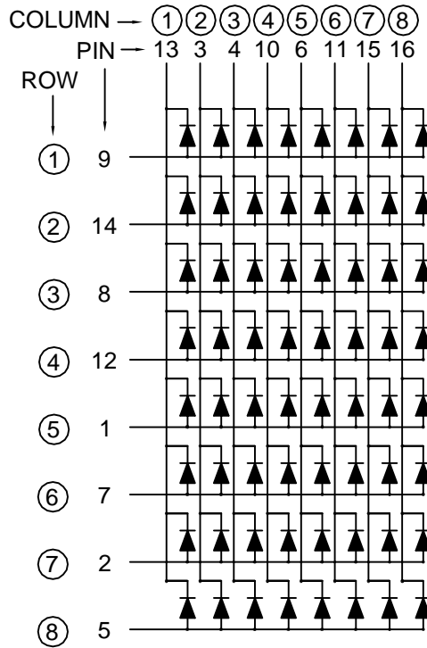
LMD8812ESR-XX-PF
