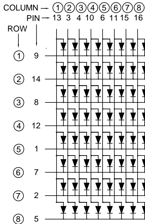
LMD8812ESR-XX-PF
