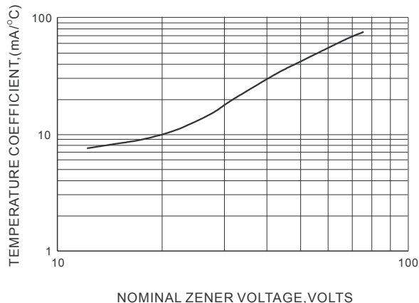
Fig. 2 TEMPERATURE COEFFICIENTS
