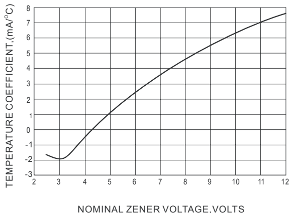
Fig. 1 TEMPERATURE COEFFICIENTS
