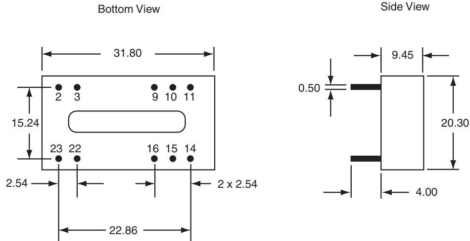
CTDD3220DF-D3K-3 Package
