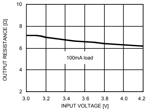
Output Resistance vs. Input Voltage (1.5x mode)
