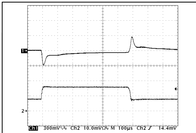
Figure 11: Output voltage response to step-change in load current (50%-100%-50% of Iout(max)). Load cap: 1µF ceramic cap and 10µF, 100 mΩ ESR tantalum cap. Ch 1: Vout (300mV/div). Ch 2: Iout (5A/div).
