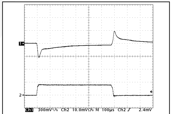
Figure 12: Output voltage response to step-change in load current (0%-50%-0% of Iout(max)). Load cap: 1µF ceramic cap and 10µF, 100 mΩ ESR tantalum cap. Ch 1: Vout (300mV/div). Ch 2: Iout (5A/div).
