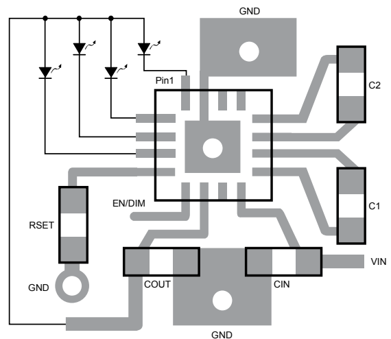
Figure 5. Recommended Layout
