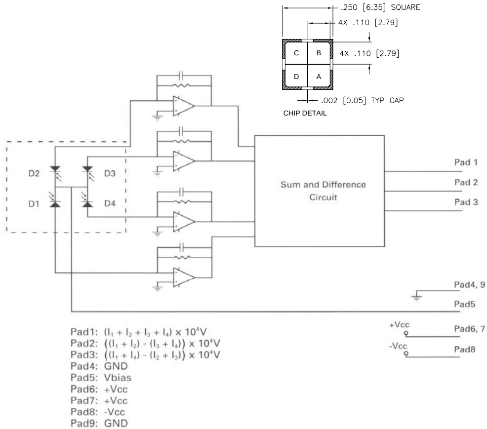
Figure 6: BPD schematic
