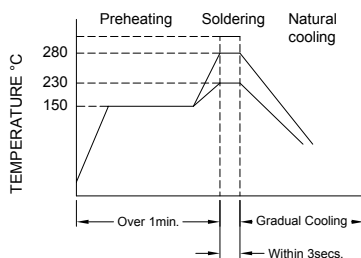
Figure 3. Hand Soldering
