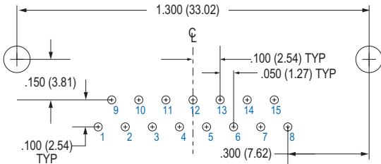
15 SOCKET M83513/19-B
