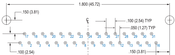
31 SOCKET M83513/19-E
