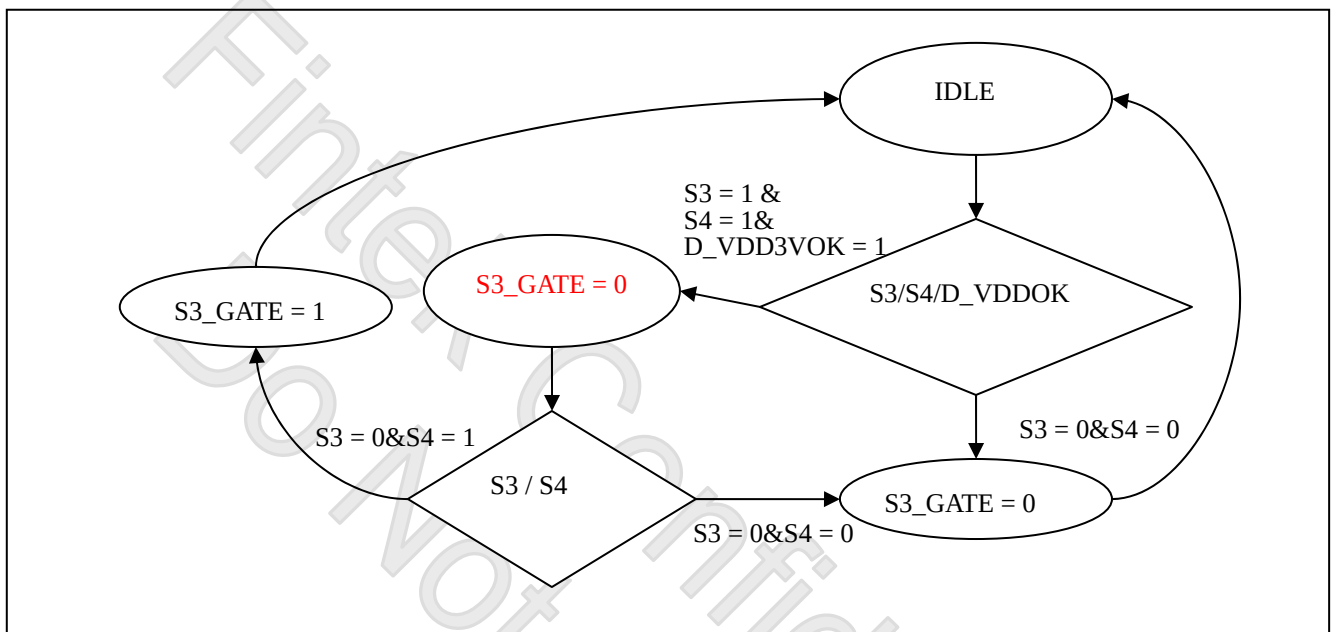
S3_GATE diagram
