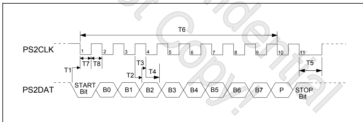
Host received from PS/2 interface timing diagram
