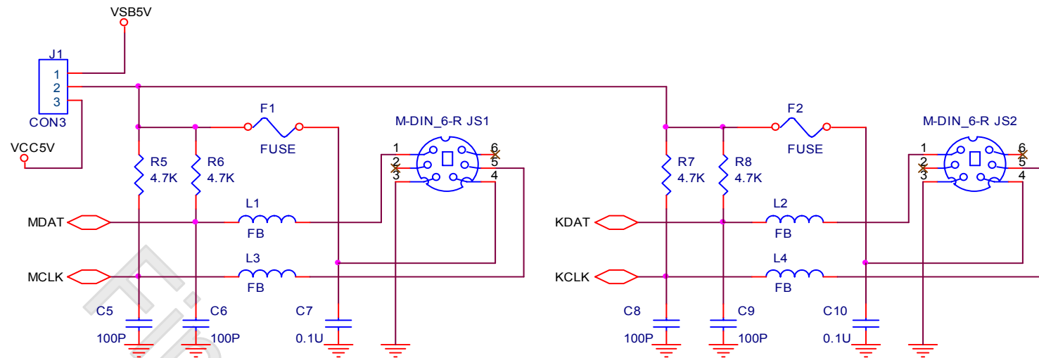
PS2 MOUSE INTERFACE
