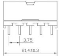
LATERAL VIEW
