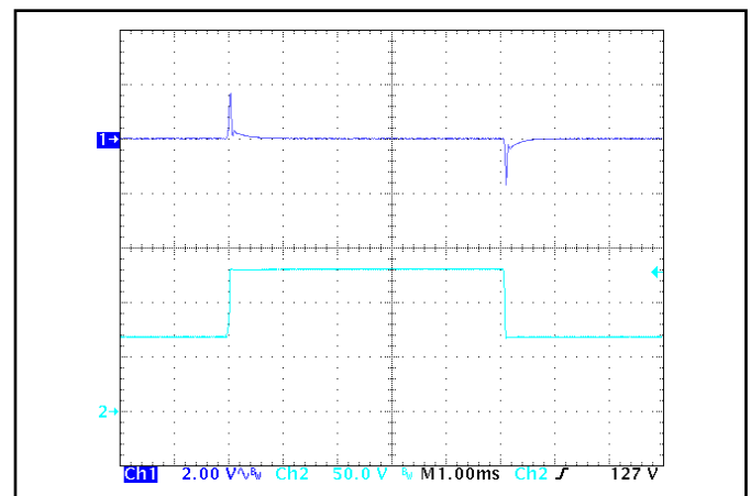
Figure 6: Output voltage response to step-change in input voltage (500 V/ms). Load cap: 100 µF, electrolytic output capacitance. Ch 1: V out (2 V/div), Ch 2: V in (50 V/div).
