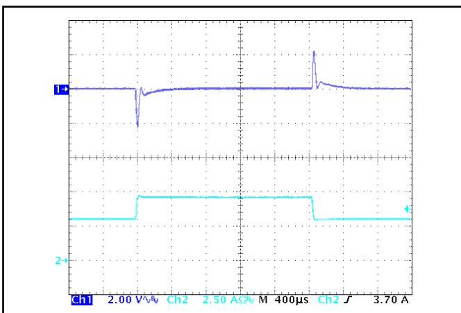
Figure 5: Output voltage response to step-change in load current (50%-75%-50% of I out (max); dl/dt = 0.1 A/μs). Load cap: 1 μF ceramic capacitor. Ch 1: V out (2 V/div), Ch 2: I out (2.5 A/div).
