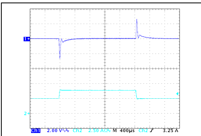
Figure 5: Output voltage response to step-change in load current (50%-75%-50% of Iout(max)); dI/dt = 0.1 A/µs. Load cap: 1 µF ceramic capacitor. Ch 1: Vout (2 V/div), Ch 2: Iout (2.5 A/div).
