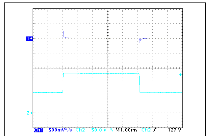
Figure 6: Output voltage response to step-change in input voltage (500 V/ms). Load cap: 100 \mu\text{F} , electrolytic output capacitance. Ch 1: Vout (500 mV/div), Ch 2: Vin (50 V/div).
