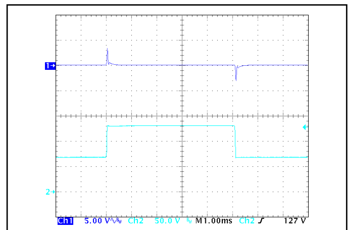
Figure 6: Output voltage response to step-change in input voltage (500 V/ms). Load cap: 100 µF, electrolytic output capacitance. Ch 1: Vout (5 V/div), Ch 2: Vin (50 V/div).
