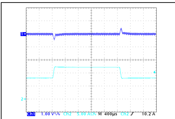
Figure 5: Output voltage response to step-change in load current (50%-75%-50% of I out (max)); dI/dt = 0.1 A/μs. Load cap: 15 μF Tantalum + 1 μF Ceramic capacitor. Ch 1: V out (1 V/div), Ch 2: I out (5 A/div).
