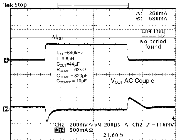
Fig. 8 Load-transient response at V_{IN}=3.3\text{V} , V_{OUT}=5\text{V}
