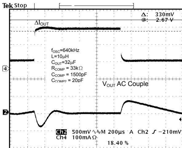
Fig. 7 Load-transient response at V_{IN}=3.3\text{V} , V_{OUT}=10\text{V}
