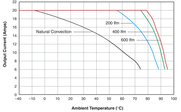
USQ-1.5/20-D48: Maximum Output Current vs. Ambient Temperature (Transverse air flow, pin 1 to pin 3; V IN = 48V, no heat sink.)
