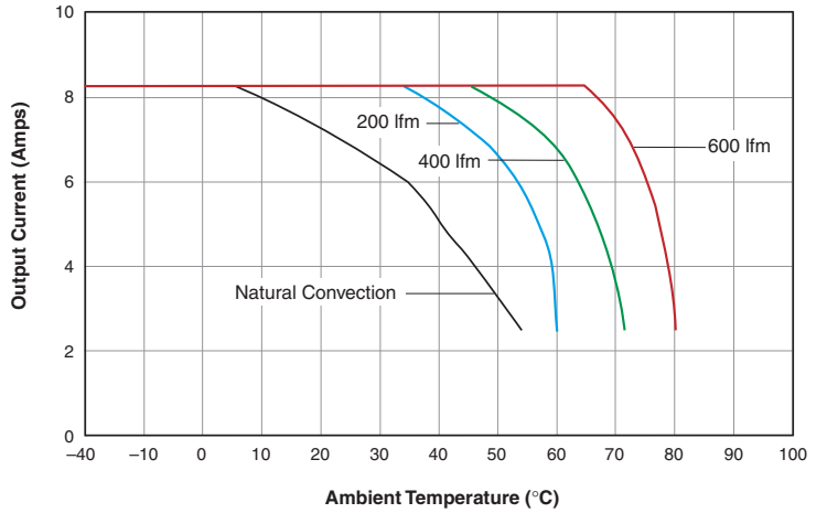
USQ-12/8.3-D48: Output Current vs. Ambient Temperature
