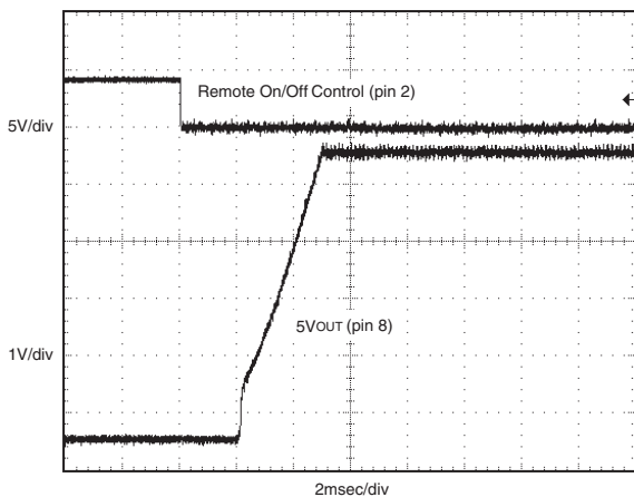
Start-Up from Remote On/Off Control (VIN = 48V, IOUT = 20A, COUT = 10µF tantalum || 1µF ceramic.)
