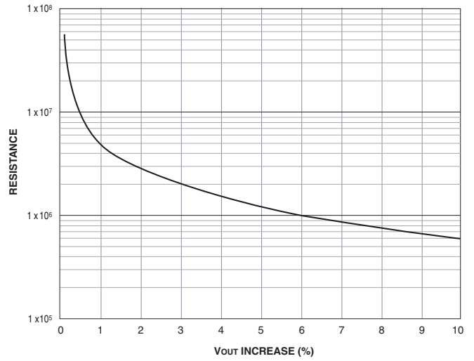
Figure 14. USQ-15 Trim-Up Resistance vs. % Increase Vout
