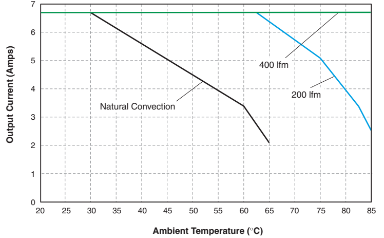
USQ-15/6.7-D48: Maximum Output Current vs. Ambient Temperature (Transverse air flow, pin 1 to pin 3; V IN = 48V, no heat sink.)
