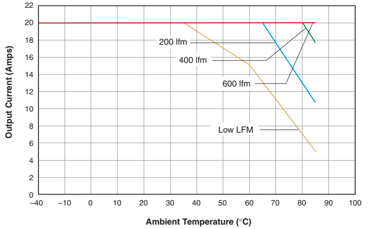
USQ-3.3/20-D48: Maximum Output Current vs. Ambient Temperature (Transverse air flow, pin 1 to pin 3; V IN = 48V, no heat sink.)
