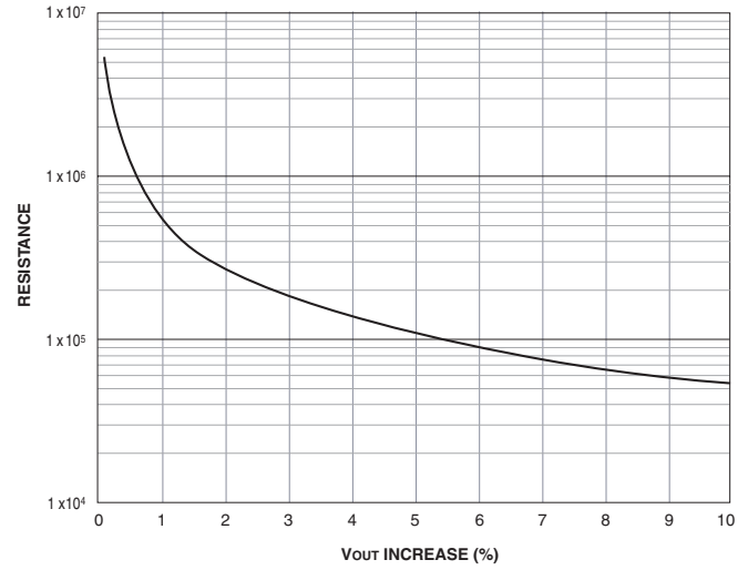
Figure 10. USQ-2.5 Trim-Up Resistance vs. % Increase Vout
