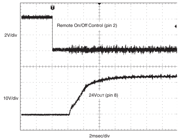
Start-Up from Remote On/Off Control
