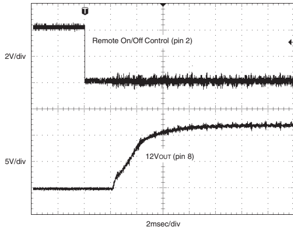
Start-Up from Remote On/Off Control (V IN = 48V, I OUT = 8.3A, C OUT = 10μF tantalum || 1μF ceramic.)
