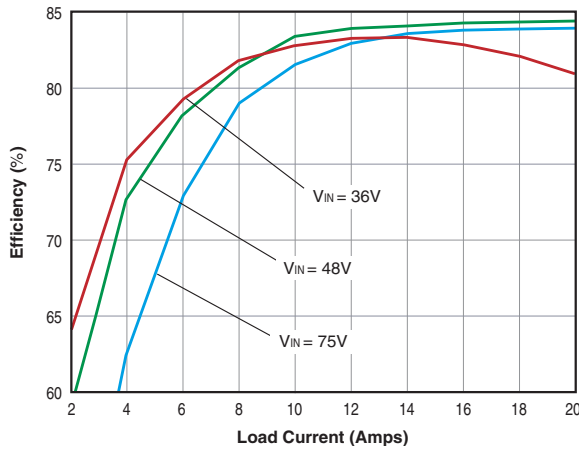
USQ-1.5/20-D48 Efficiency vs. Line Voltage/Load Current @ 25°C
