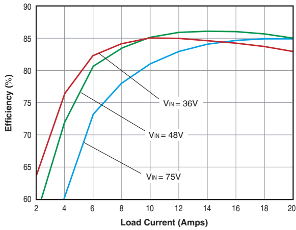
USQ-1.8/20-D48 Efficiency vs. Line Voltage/Load Current @ 25°C
