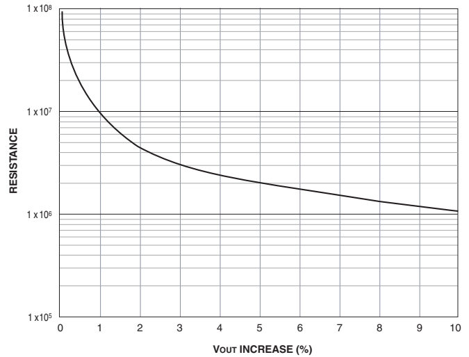
Figure 16. USQ-24 Trim-Up Resistance vs. % Increase Vout
