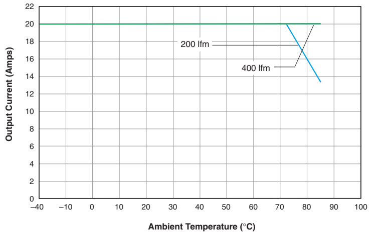
USQ-3.3/20-D48: Maximum Output Current vs. Ambient Temperature (Longitudinal air flow, pin 1 to pin 3; V IN = 48V, 1/4" heat sink.)
