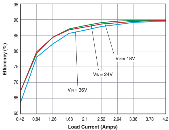
USQ-24/4.2-D24 Efficiency vs. Line Voltage/Load Current @ 25°C
