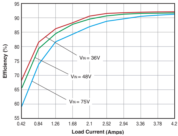
USQ-24/4.2-D48 Efficiency vs. Line Voltage/Load Current @ 25°C
