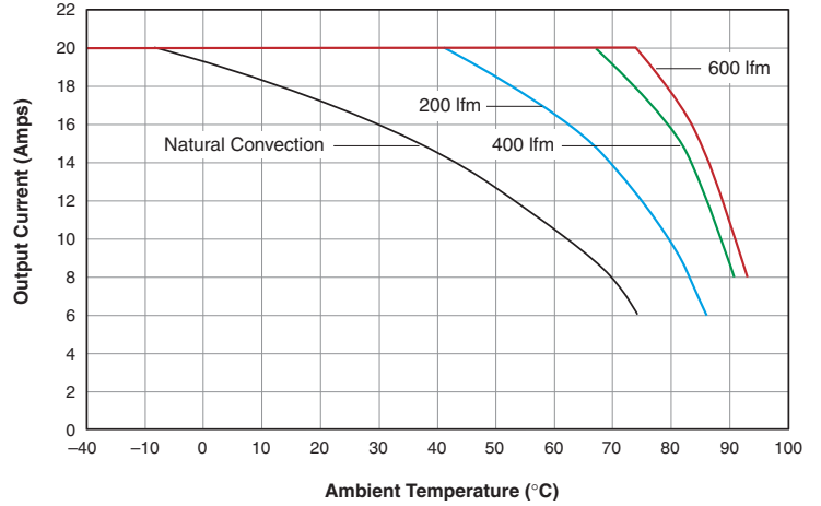
USQ-1.5/20-D48: Maximum Output Current vs. Ambient Temperature (Longitudinal air flow, pin 1 to pin 4; V IN = 48V, no heat sink.)
