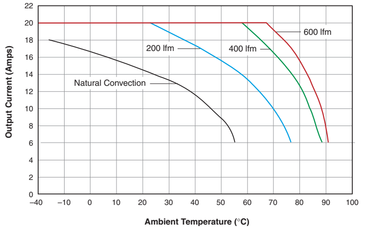
USQ-3.3/20-D48: Maximum Output Current vs. Ambient Temperature (Longitudinal air flow, pin 1 to pin 4; V IN = 48V, no heat sink.)
