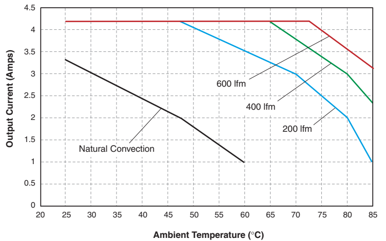
USQ-24/4.2-D24: Maximum Output Current vs. Ambient Temperature (Transverse air flow, pin 1 to pin 3; V IN = 24V, no heat sink.)
