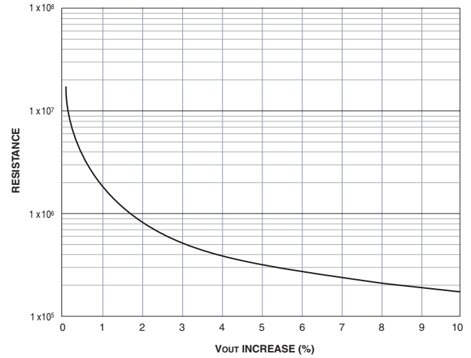
Figure 12. USQ-5 Trim-Up Resistance vs. % Increase Vout
