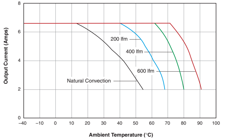
USQ-15/6.7-D48: Maximum Output Current vs. Ambient Temperature (Longitudinal air flow, pin 1 to pin 3; V IN = 48V, no heat sink.)
