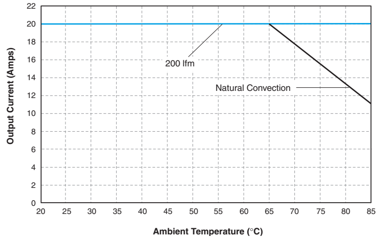
USQ-1.2/20-D48: Maximum Output Current vs. Ambient Temperature (Transverse air flow, pin 1 to pin 3; V IN = 48V, no heat sink.)
