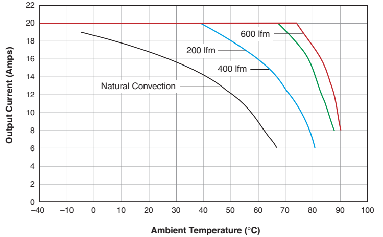
USQ-1.8/20-D48: Maximum Output Current vs. Ambient Temperature (Longitudinal air flow, pin 1 to pin 4; V IN = 48V, no heat sink.)
