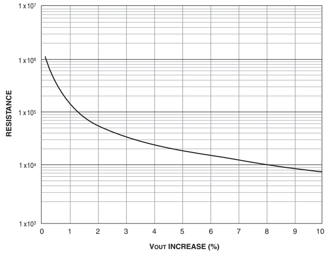
Figure 8. USQ-1.5 Trim-Up Resistance vs. % Increase Vout
