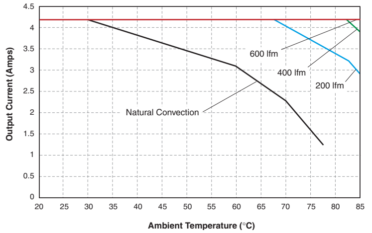
USQ-24/4.2-D48: Maximum Output Current vs. Ambient Temperature (Transverse air flow, pin 1 to pin 3; V IN = 48V, no heat sink.)
