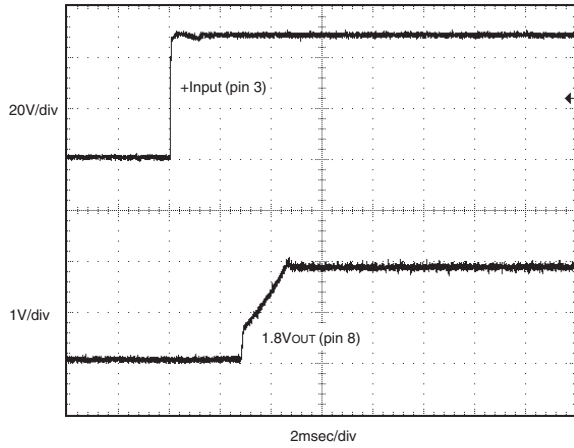
Start-Up from V IN (V IN = 48V, I OUT = 20A, C OUT = 10µF tantalum || 1µF ceramic.)
