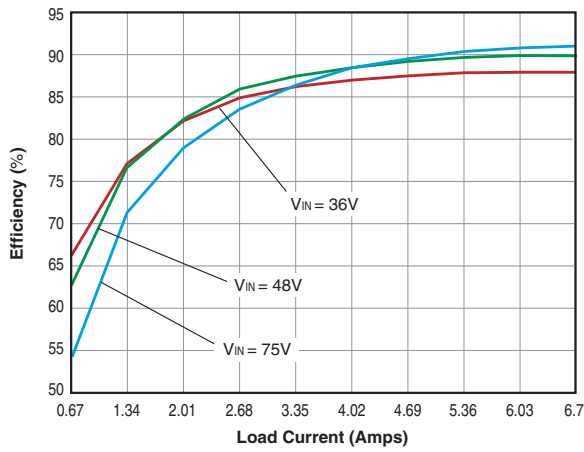
USQ-15/6.7-D48 Efficiency vs. Line Voltage/Load Current @ 25°C
