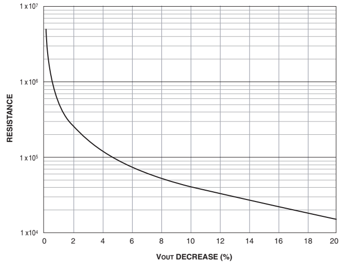
Figure 18. USQ-1.5 to USQ-18 Trim-Down Resistance vs. % Decrease Vout
