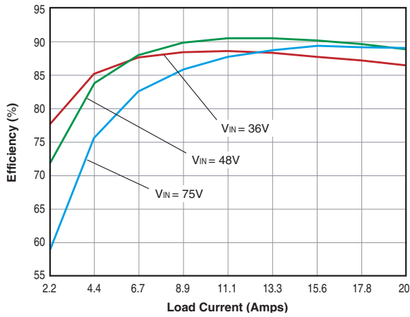
USQ-3.3/20-D48 Efficiency vs. Line Voltage/Load Current @ 25°C
