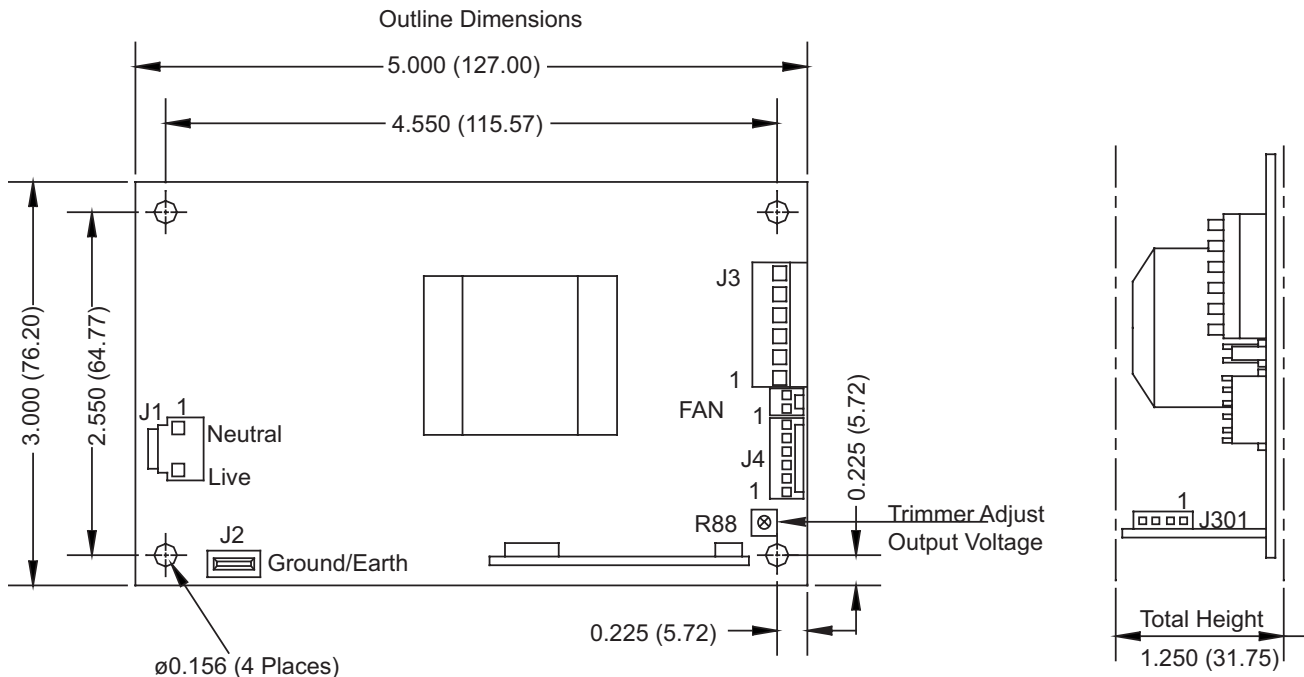
Figure 2: Mechanical Drawing
