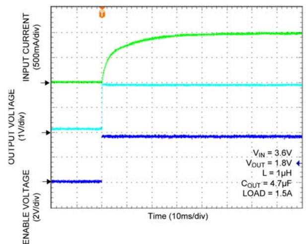
Start-Up Waveform
