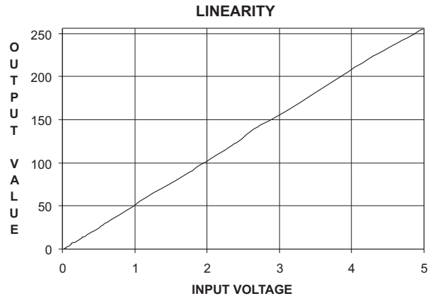
Figure 3. Measured Linearity
