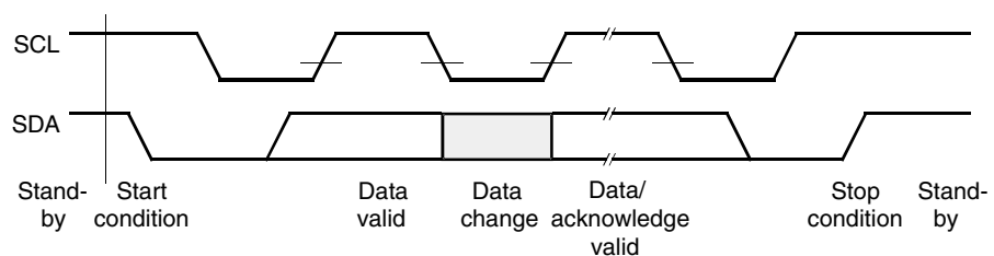
Figure 3-5. Serial Protocol
