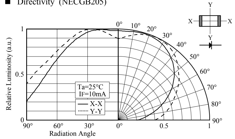
■ Directivity (NECGB205)
