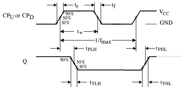
Figure 1. Switching Waveforms
