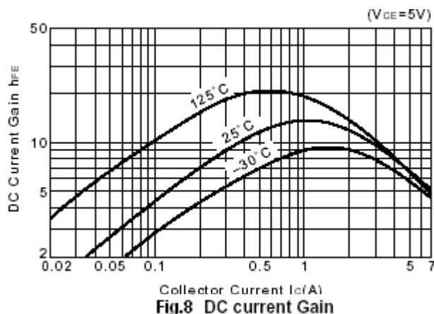
Fig.8 DC current Gain
