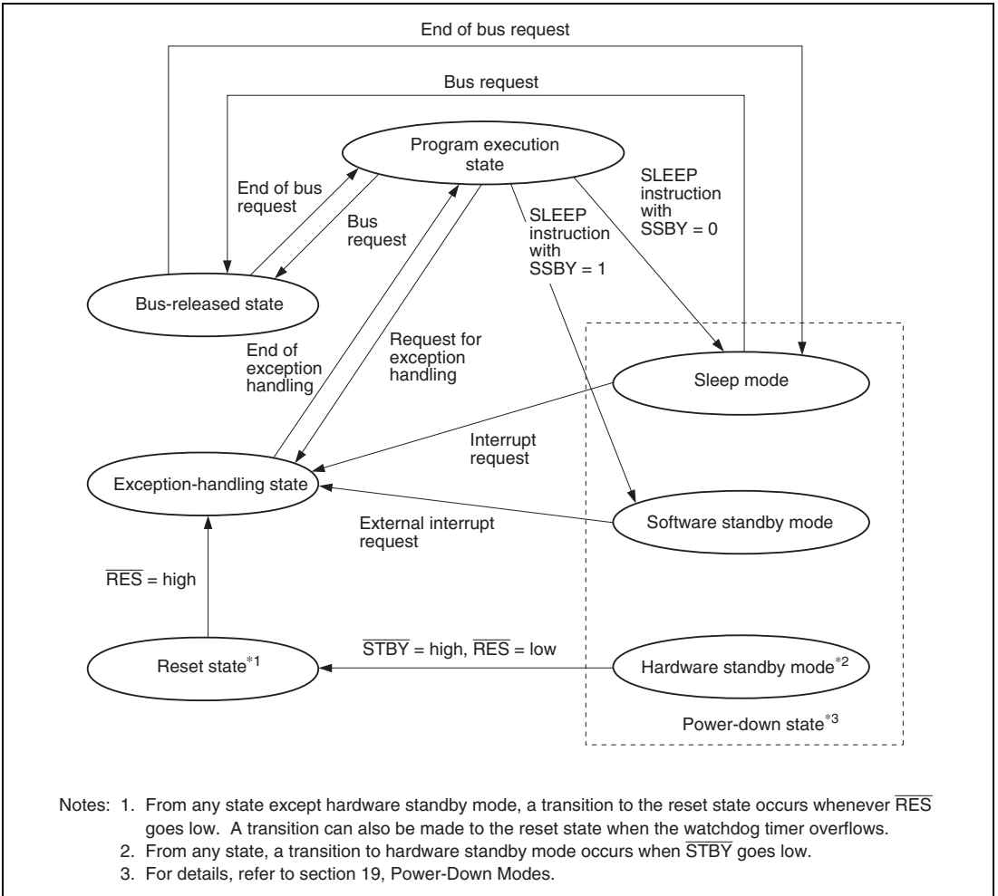
Figure 2.13 State Transitions
