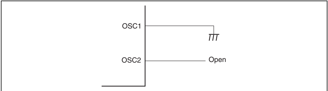
Figure 18.8 Pin Handling when Subclock is not Used
