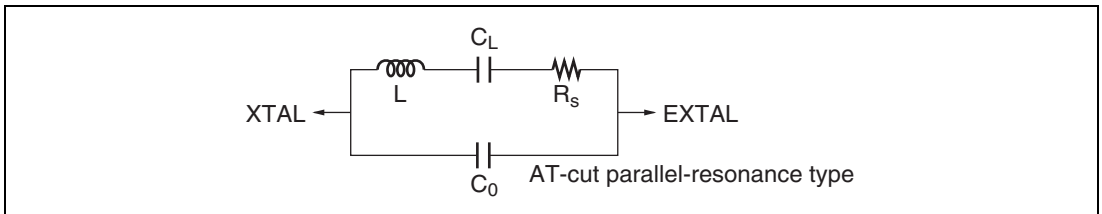
Figure 18.3 Crystal Resonator Equivalent Circuit
