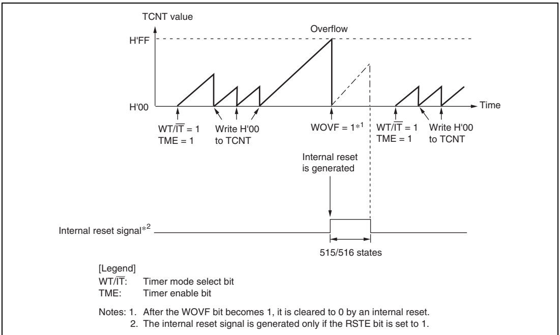
Figure 12.3 (b) WDT_1 Operation in Watchdog Timer Mode
