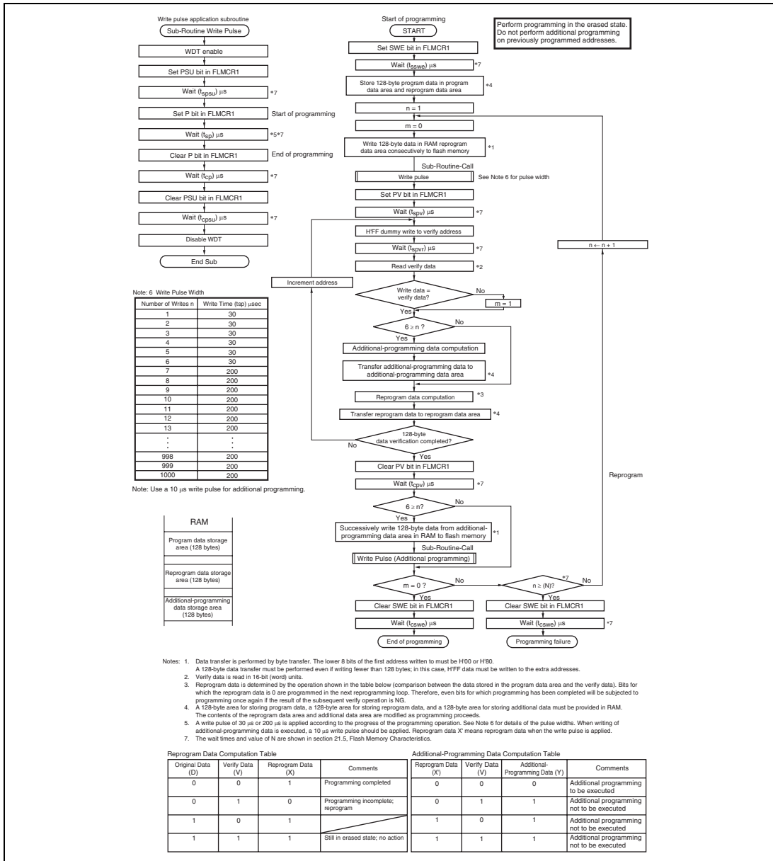
Figure 17.9 Program/Program-Verify Flowchart
