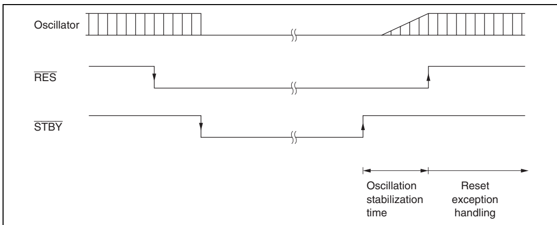
Figure 19.4 Hardware Standby Mode Timing
