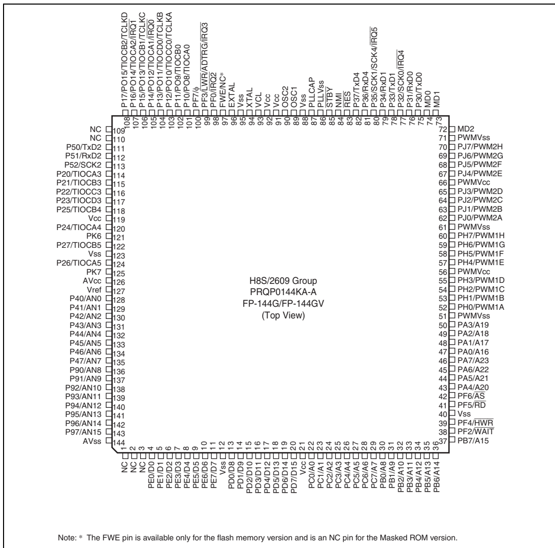
Figure 1.2 Pin Assignments
