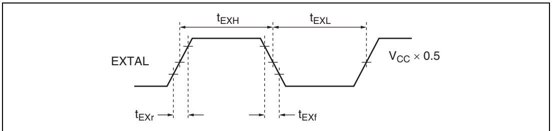
Figure 18.5 External Clock Input Timing
