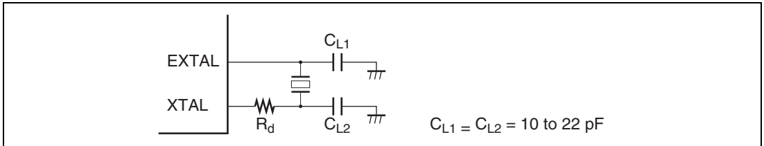
Figure 18.2 Connection of Crystal Resonator (Example)
