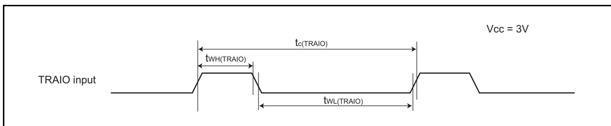
Figure 21.13 TRAIO Input Timing Diagram when V_{CC} = 3\text{ V}
