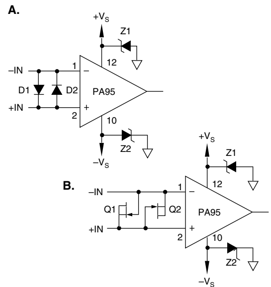
FIGURE 1. OVERVOLTAGE PROTECTION
