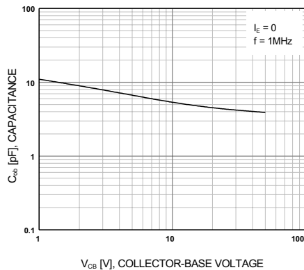
Figure 3. Output Capacitance
