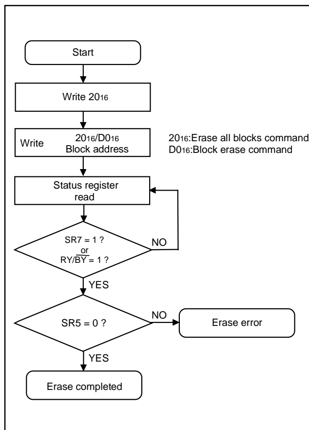
Fig. 92 Erase flowchart
