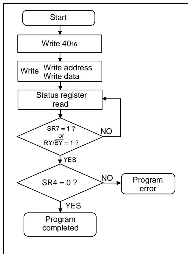
Fig. 91 Program flowchart
