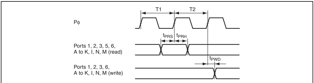
Figure 29.42 I/O Port Input/Output Timing
