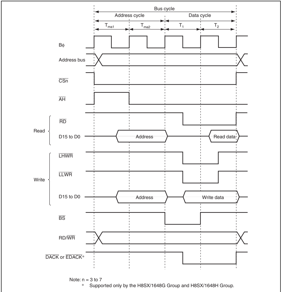
Figure 9.32 16-Bit Access Space Access Timing (ABWHn = 0, ABWLn = 1)
