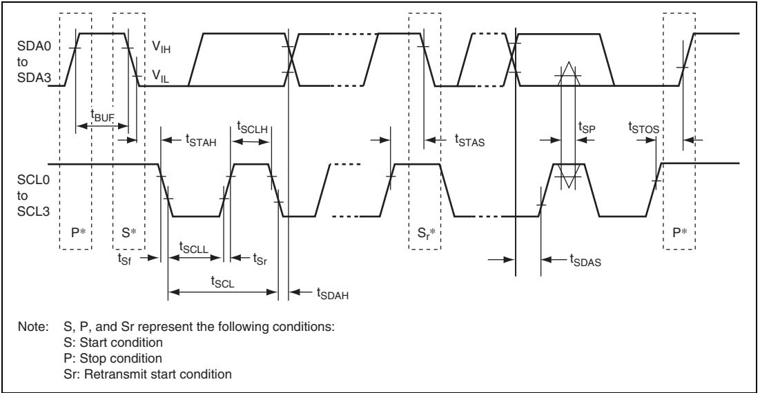
Figure 29.53 I 2 C Bus Interface 2 Input/Output Timing (Option)
