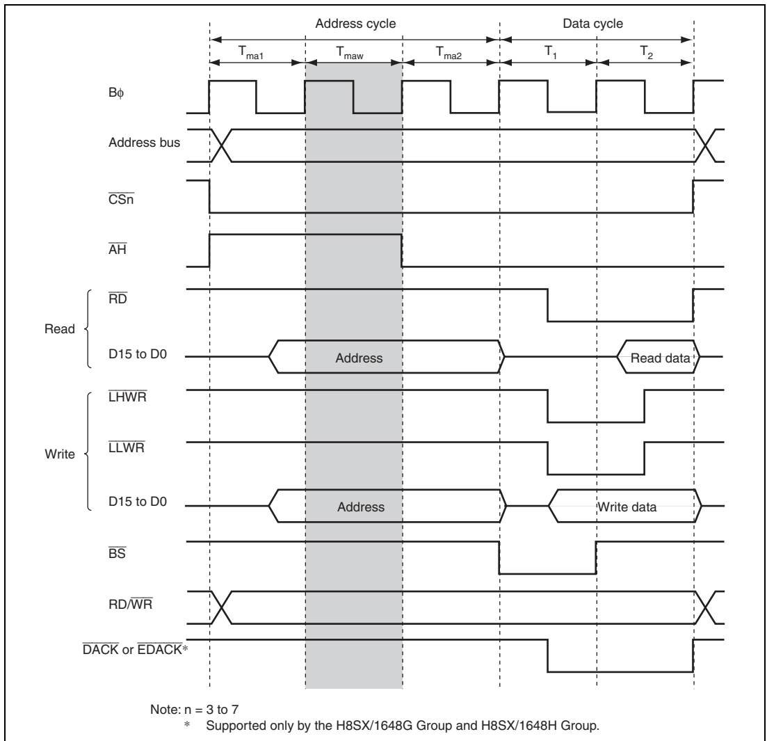
Figure 9.33 Access Timing of 3 Address Cycles (ADDEX = 1)
