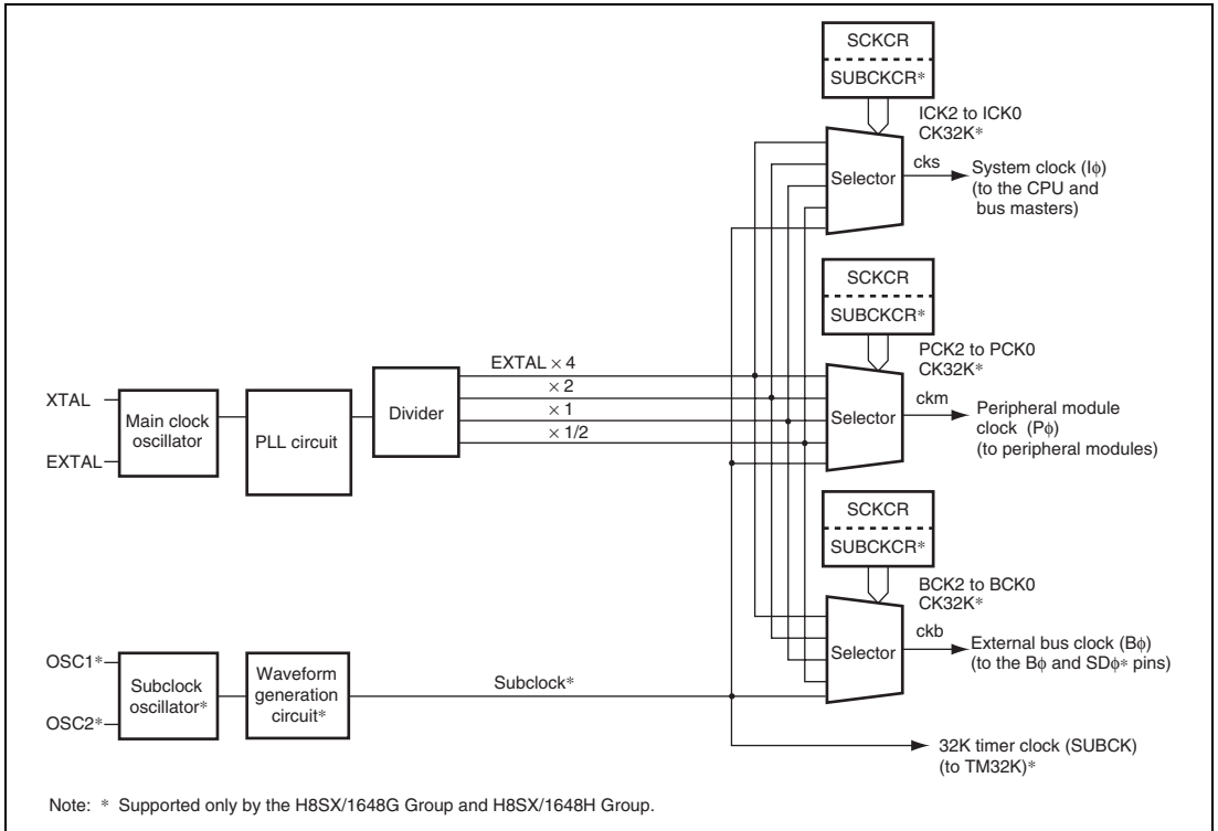
Figure 26.1 Block Diagram of Clock Pulse Generator
