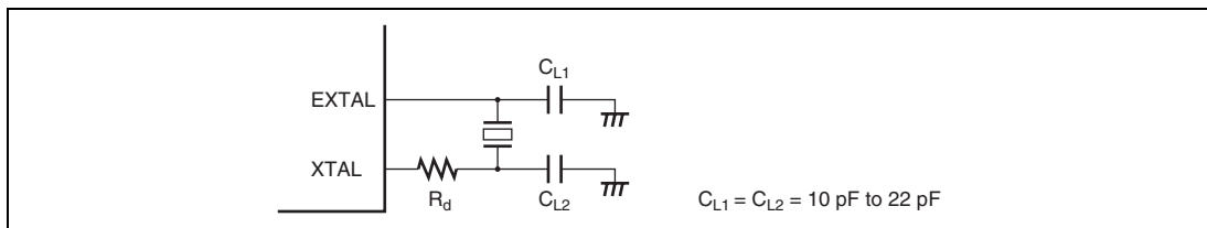
Figure 26.2 Connection of Crystal Resonator (Example)
