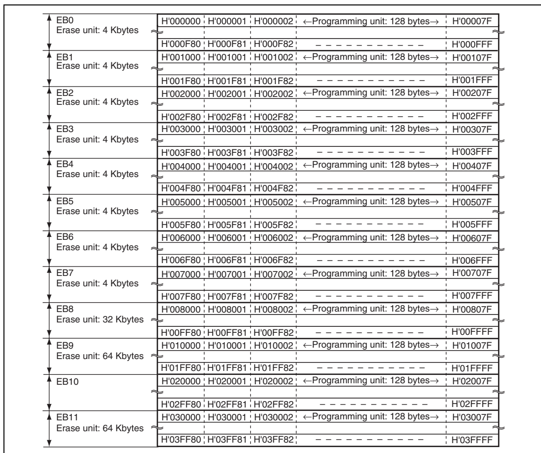
Figure 24.4 User MAT Block Structure of H8SX/1642
