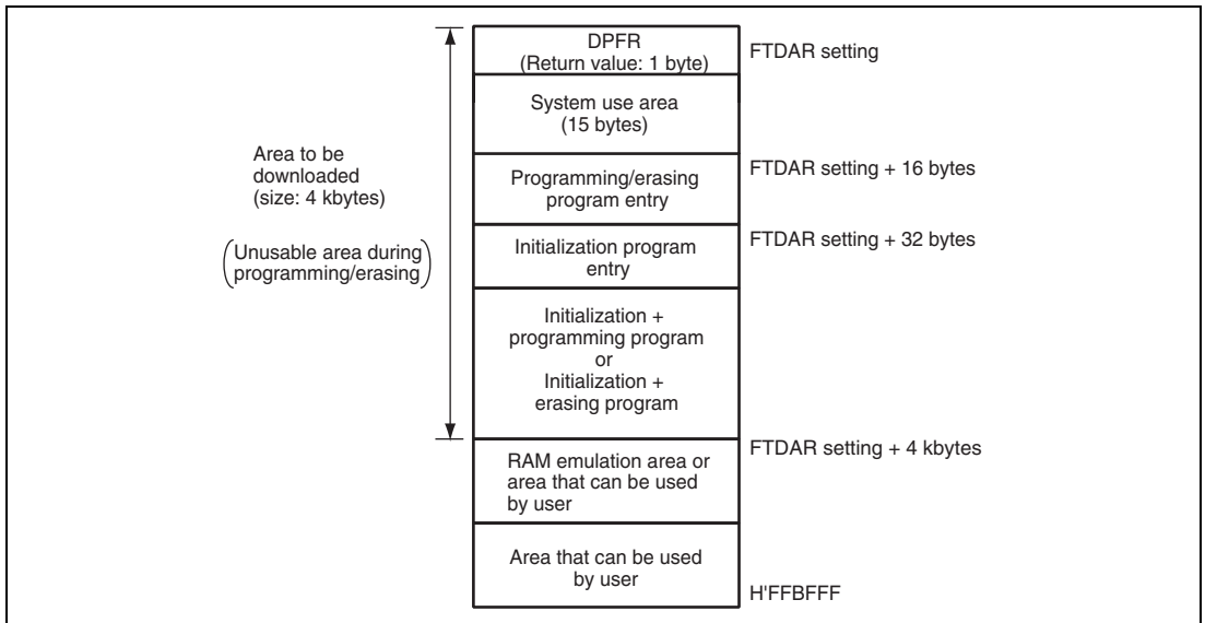
Figure 24.10 RAM Map when Programming/Erase is Executed
