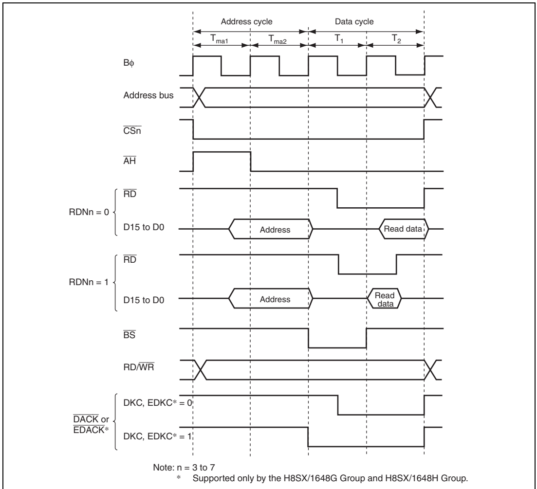
Figure 9.37 Output Timing for \overline{\text{DACK}} and \overline{\text{EDACK}}^* Signals
