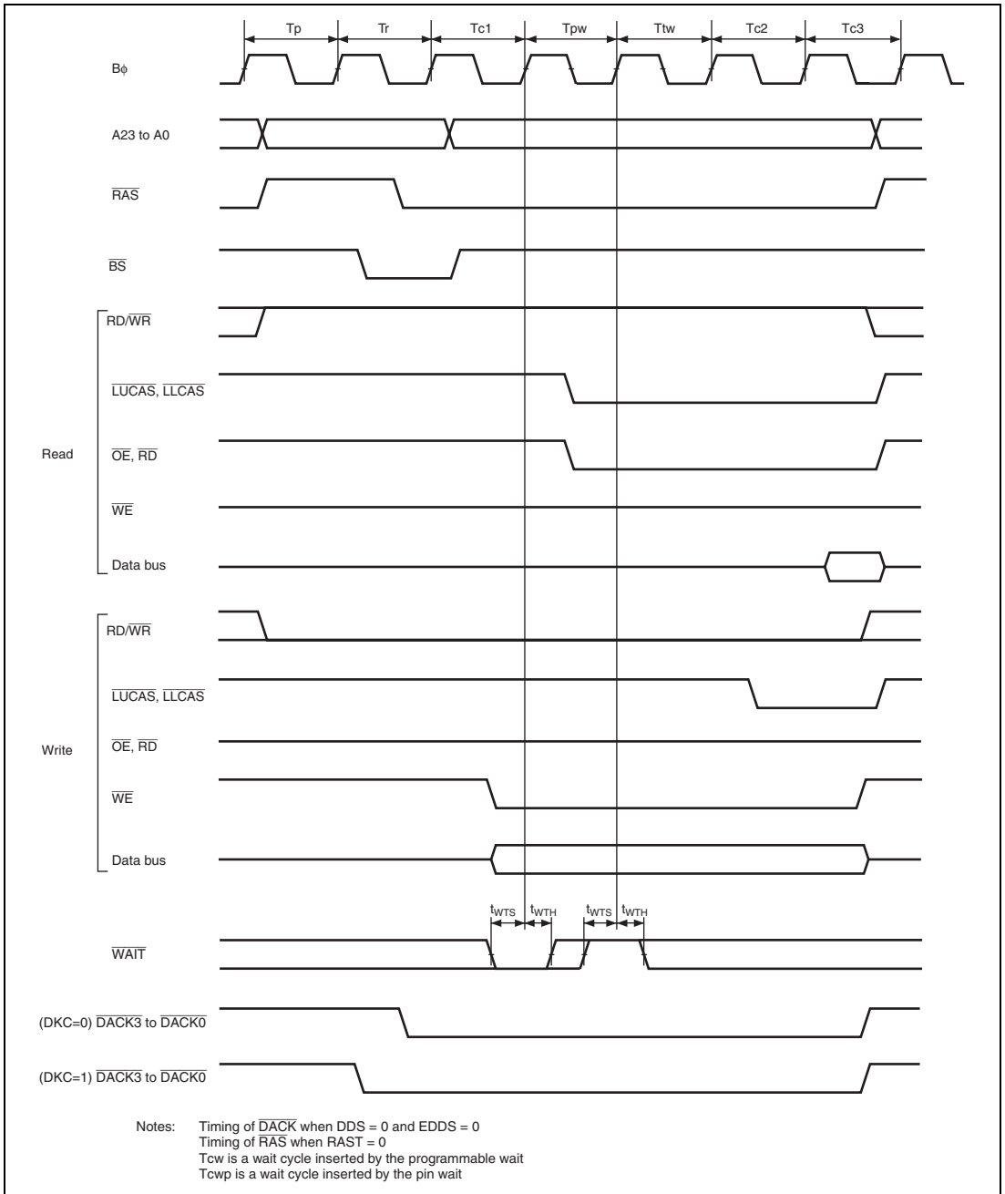
Figure 29.23 DRAM Access Timing / Three-State Access, One Wait*
