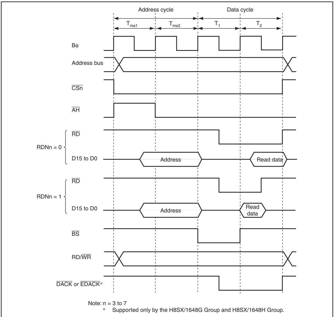
Figure 9.34 Read Strobe Timing
