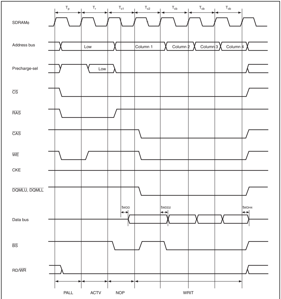
Figure 29.33 Synchronous DRAM Cluster Transfer Access Timing (Write)*
