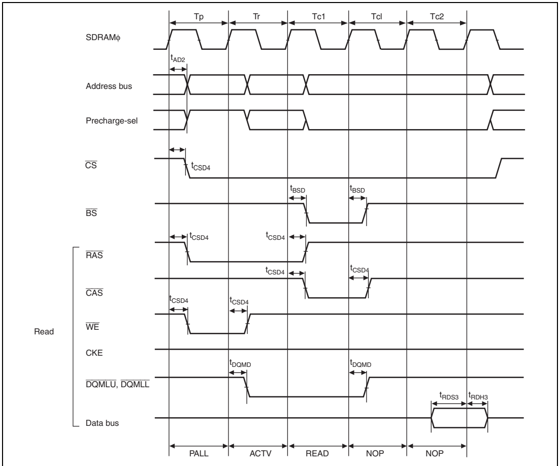
Figure 29.29 Synchronous DRAM Basic Read Access Timing (CAS Latency 2)*
