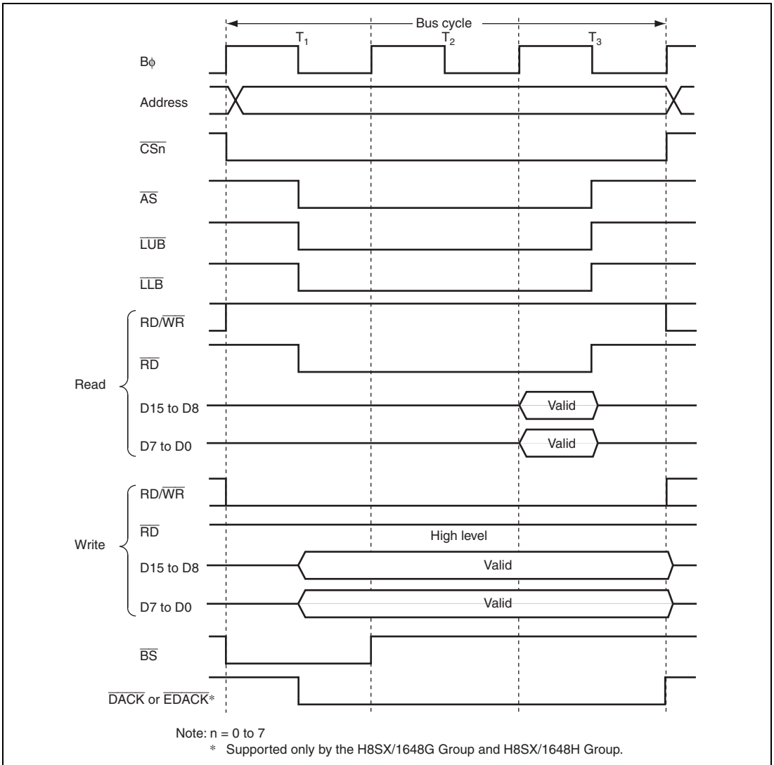
Figure 9.26 16-Bit 3-State Access Space Bus Timing
