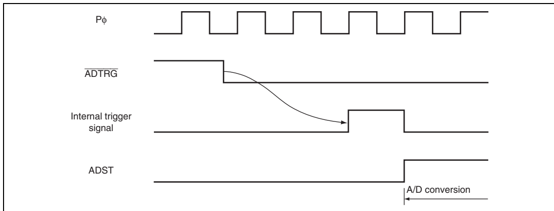
Figure 21.8 External Trigger Input Timing (TRGS1, TRGS0, and EXTRGS ≠ B'111)
