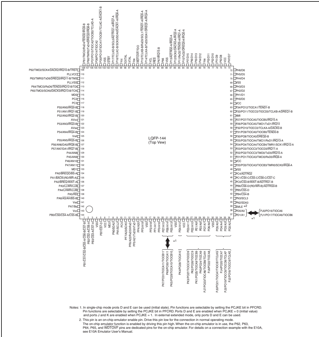
Figure 1.3 Pin Assignments (LQFP-144: H8SX/1648, 1648A, and 1648L Groups)
