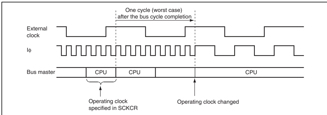
Figure 26.9 Clock Modification Timing
