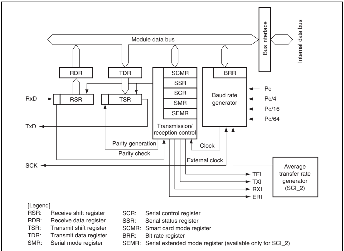
Figure 19.1 Block Diagram of SCI_0, 1, 2, 3, and 4
