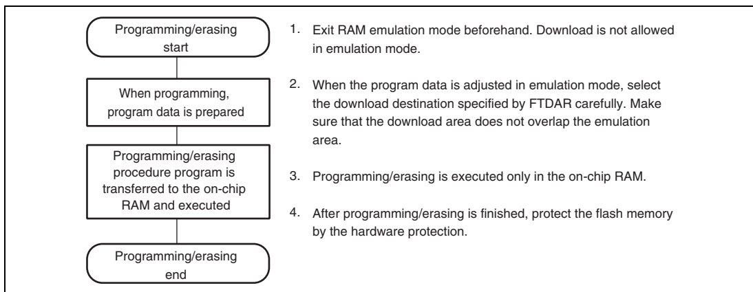
Figure 24.9 Programming/Erasing Flow
