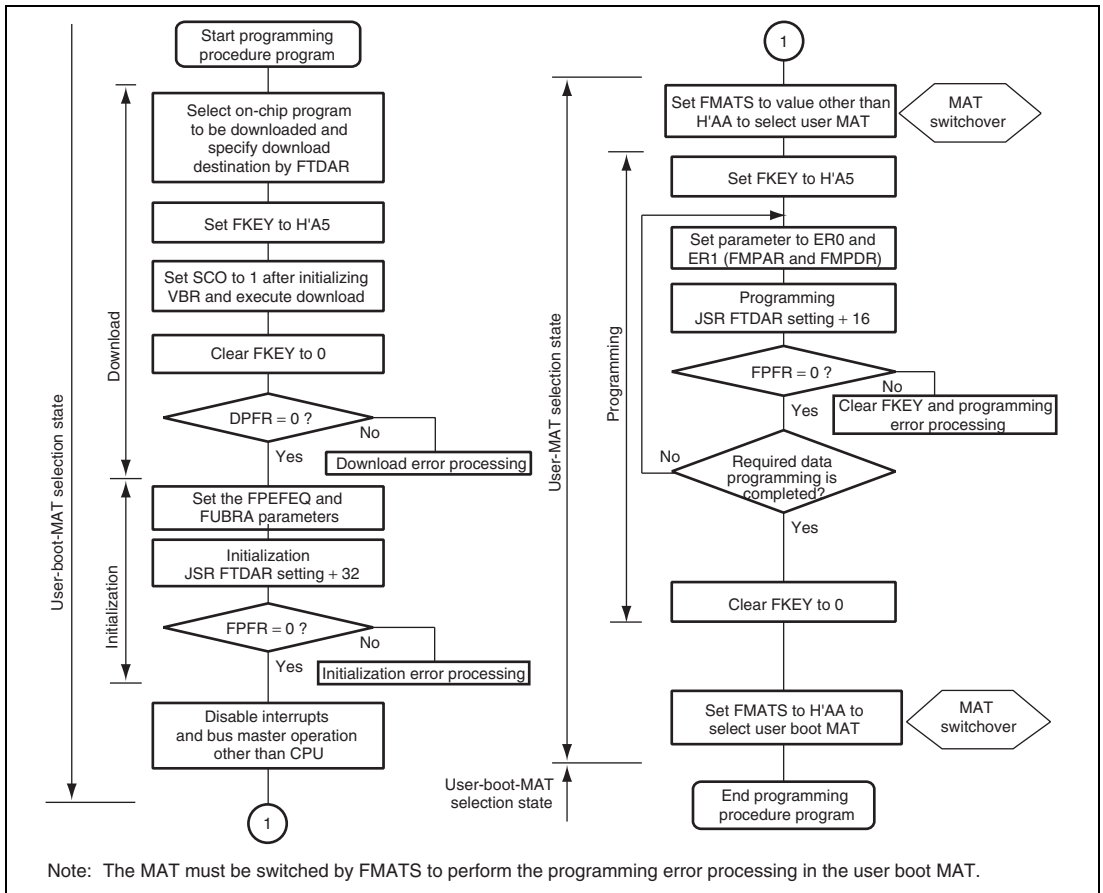
Figure 24.14 Procedure for Programming User MAT in User Boot Mode
