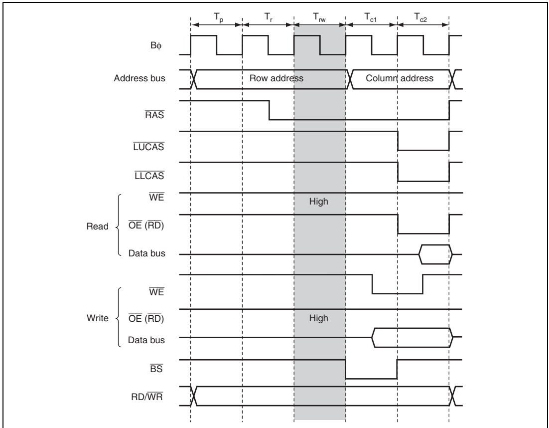
Figure 9.41 Access Timing Example when One T_{rw} Cycle is Specified ( RAS\#=0 , CAS\#=0 )
