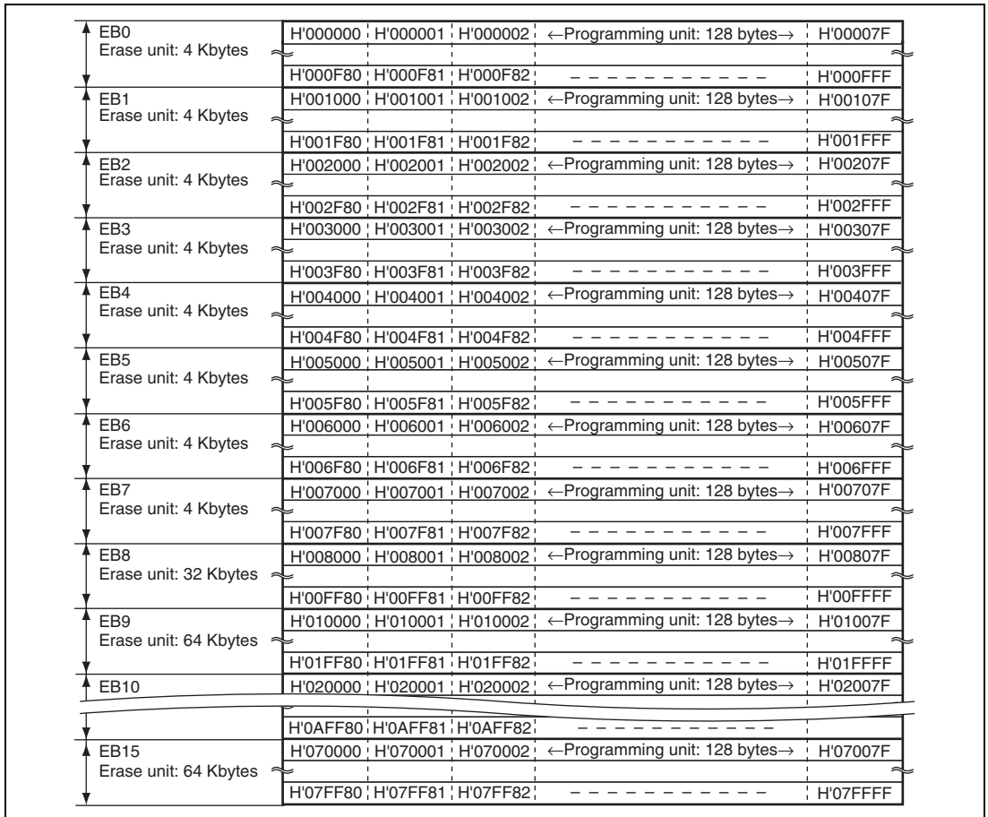
Figure 24.4 User MAT Block Structure of H8SX/1644
