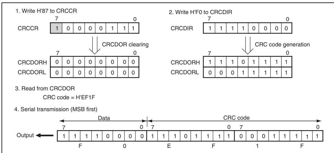
Figure 19.45 MSB-First Data Transmission
