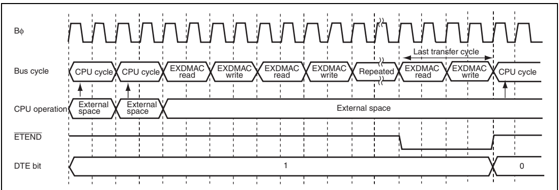
Figure 11.41 Auto-Request/Normal Transfer Mode/Burst Mode (CPU Cycles/Dual Address Mode)
