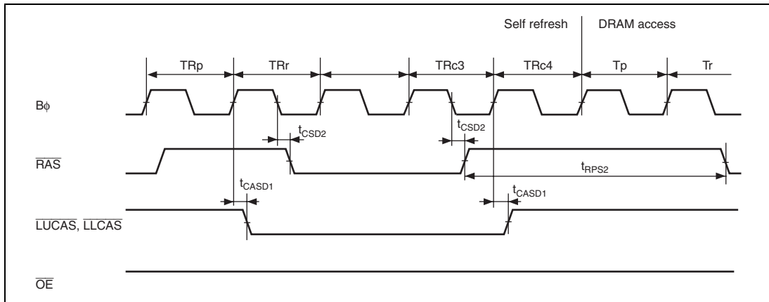
Figure 29.27 Self-Refresh Timing (After Leaving Software Standby: RAST=0)*
