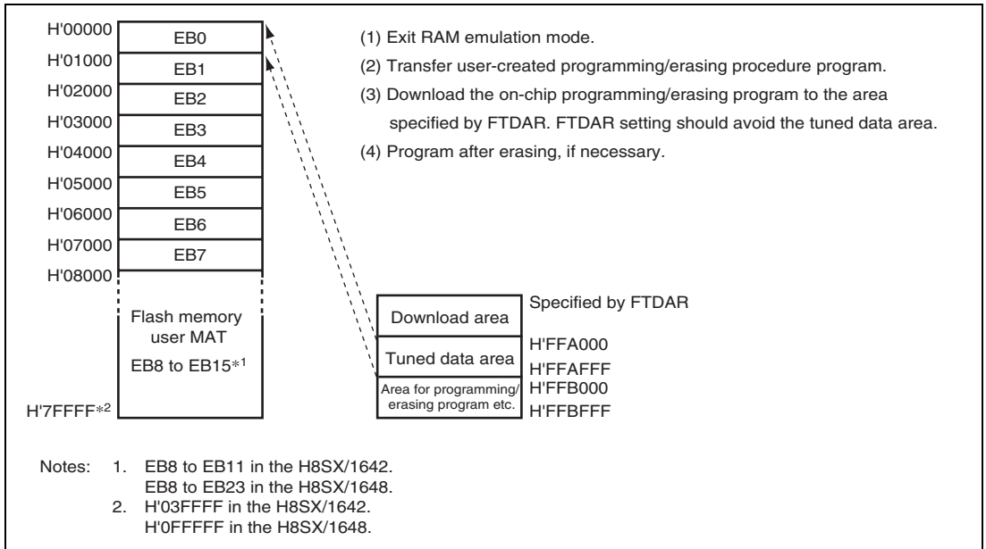
Figure 24.19 Programming Tuned Data (H8SX/1644)
