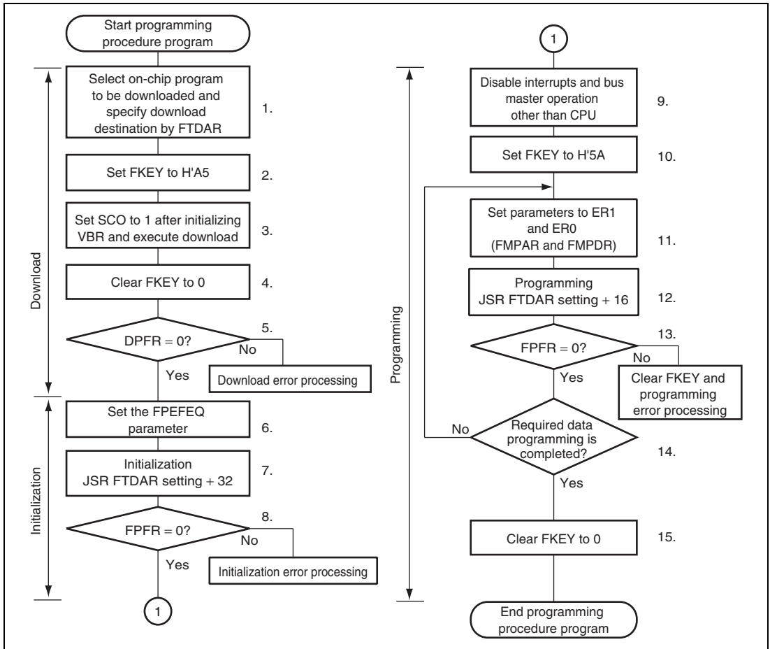
Figure 24.11 Programming Procedure in User Program Mode
