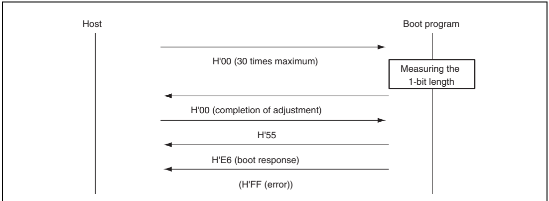
Figure 24.22 Bit-Rate-Adjustment Sequence
