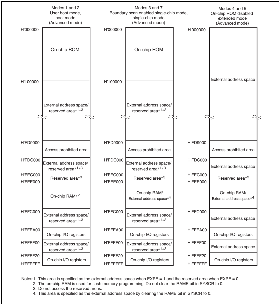
Figure 3.1 Address Map in Each Operating Mode of H8SX/1648, 1648A, 1648L, 1648G, and 1648H (1)
