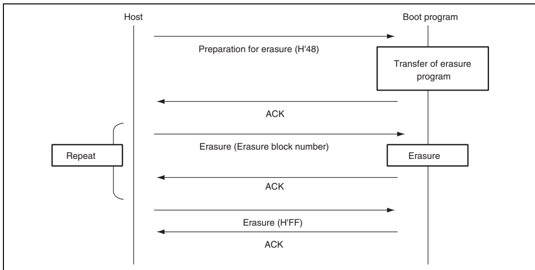
Figure 24.26 Erasure Sequence
