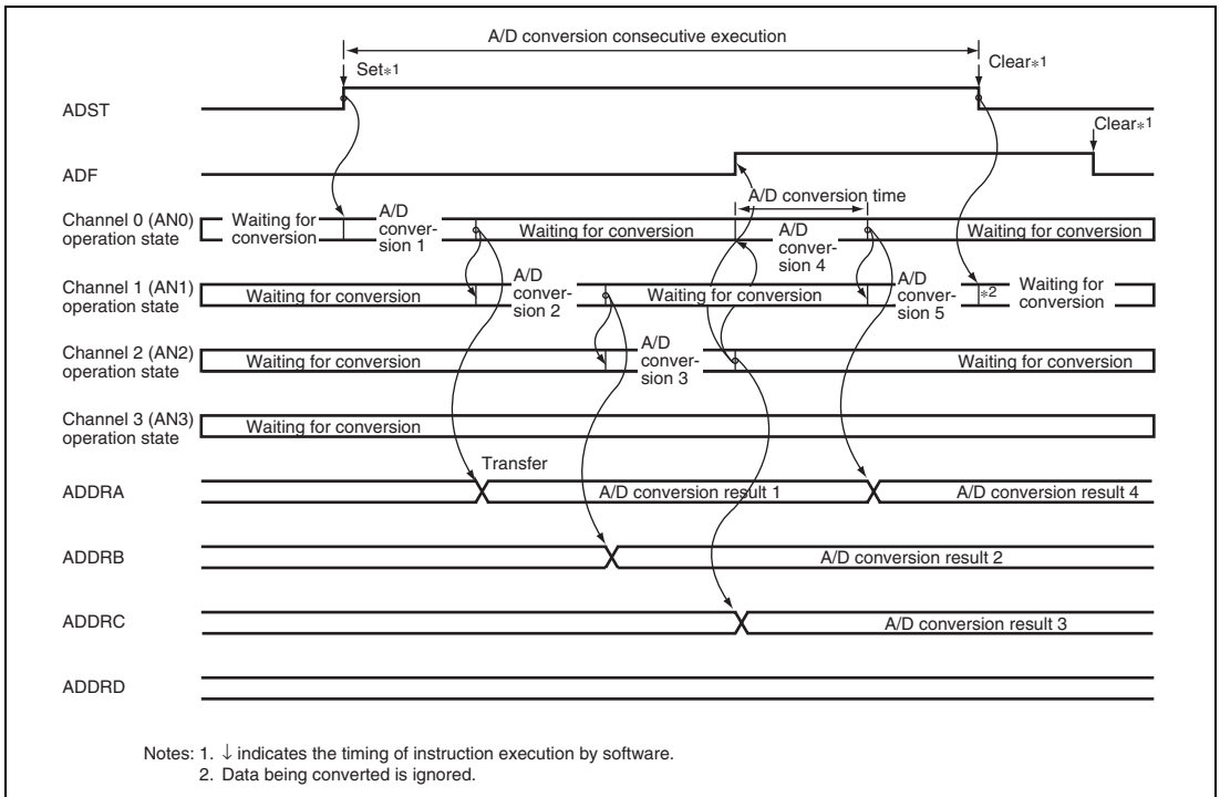
Figure 21.5 Example of A/D Conversion (Continuous Scan Mode, Three Channels (AN0 to AN2) Selected)
