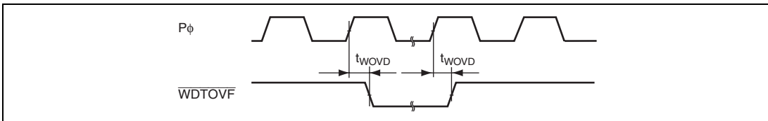
Figure 29.49 WDT Output Timing
