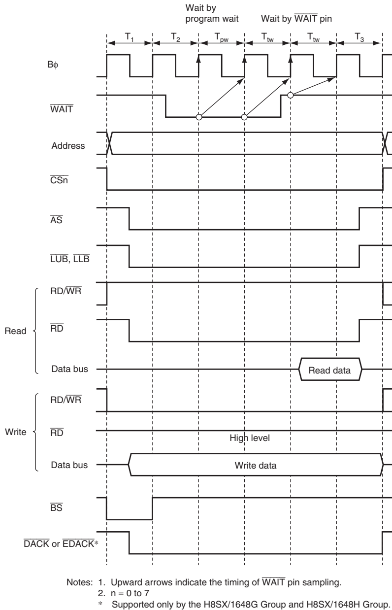
Figure 9.27 Example of Wait Cycle Insertion Timing
