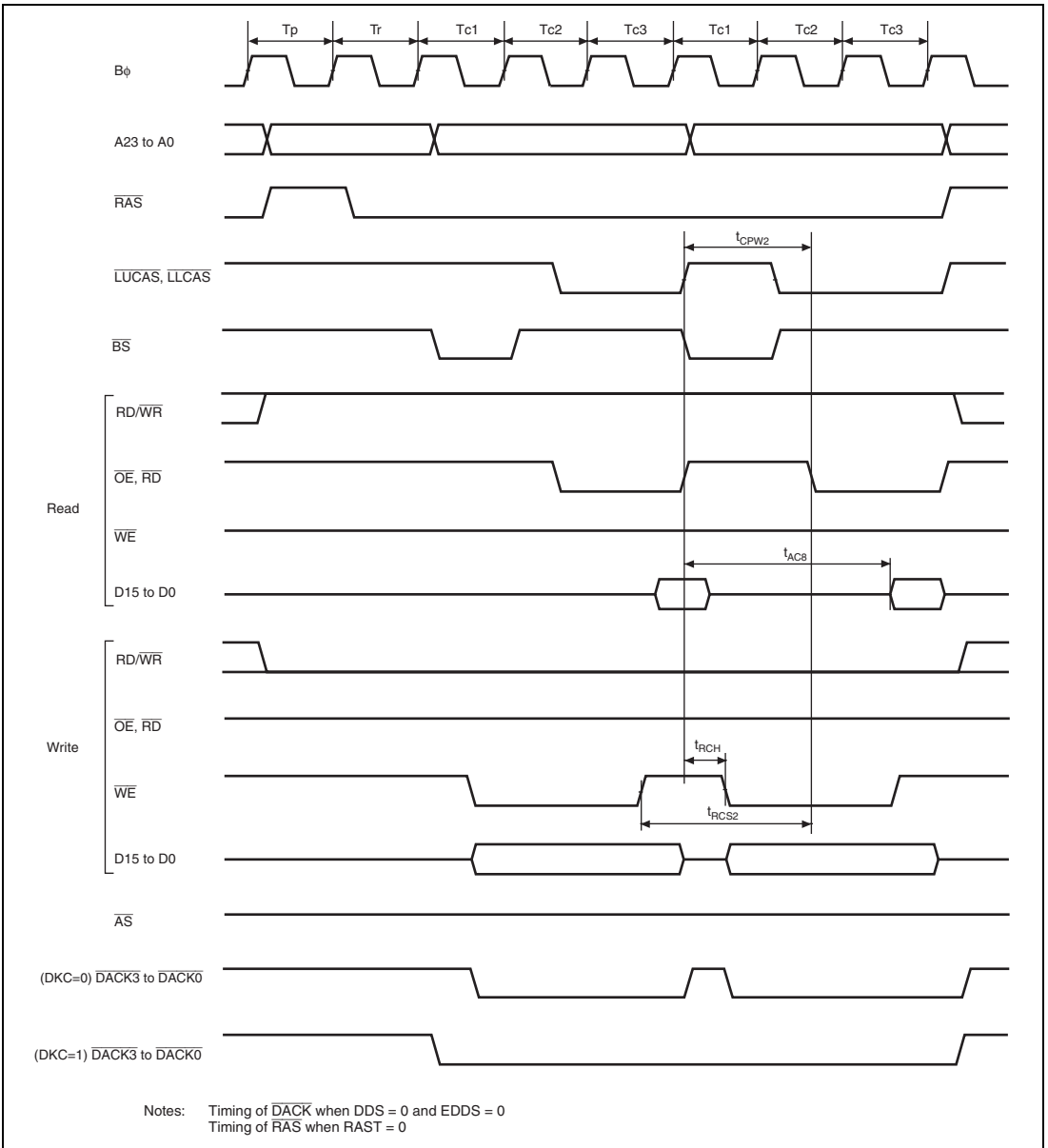
Figure 29.24 DRAM Access Timing / Three-State Burst Access*
