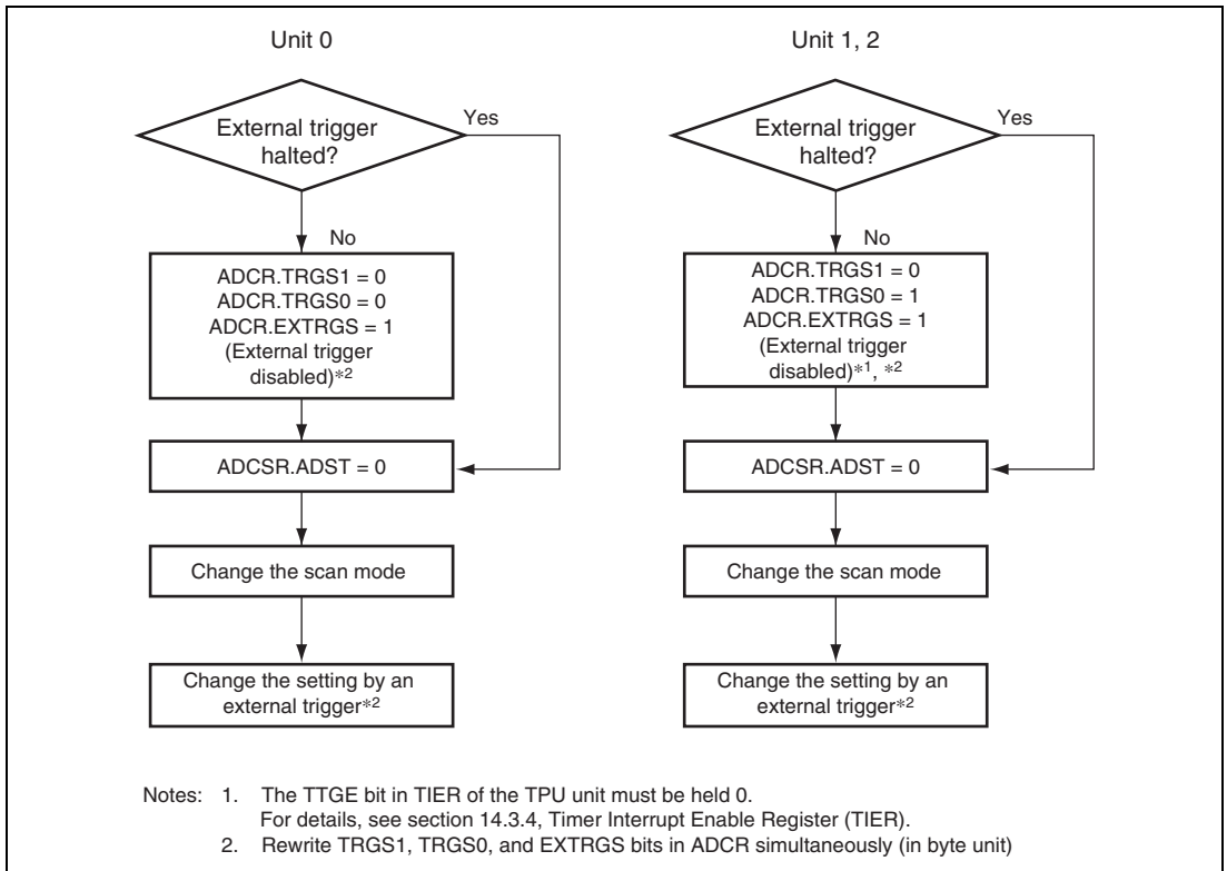
Figure 21.12 Procedure for Changing the Mode When the Setting for Activation by an External Trigger is in Use
