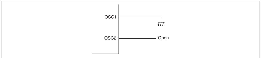
Figure 26.8 Pin Handling when Subclock is not Used
