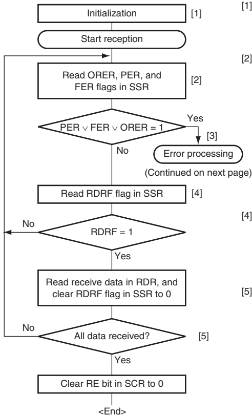
Figure 19.12 Sample Serial Reception Flowchart (1)
