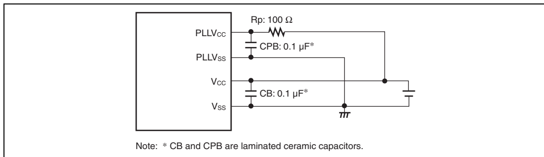
Figure 26.11 Recommended External Circuitry for PLL Circuit
