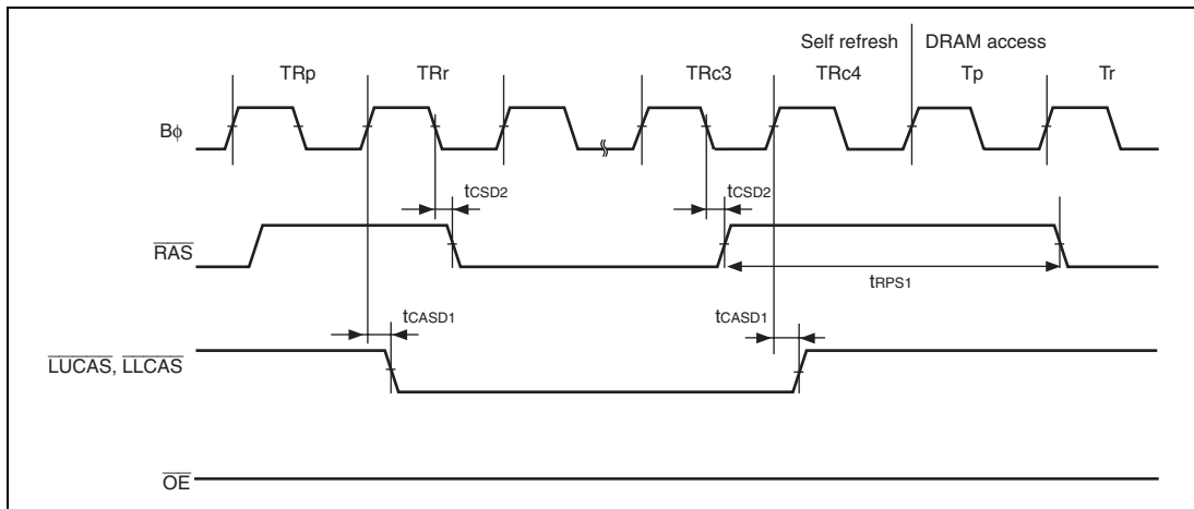
Figure 29.28 Self-Refresh Timing (After Leaving Software Standby: RAST=1)*
