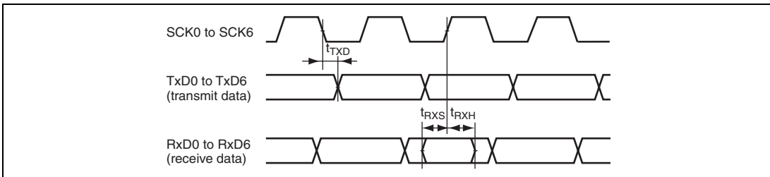
Figure 29.51 SCI Input/Output Timing: Clocked Synchronous Mode
