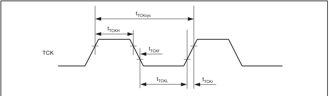
Figure 29.54 Boundary Scan TCK Timing
