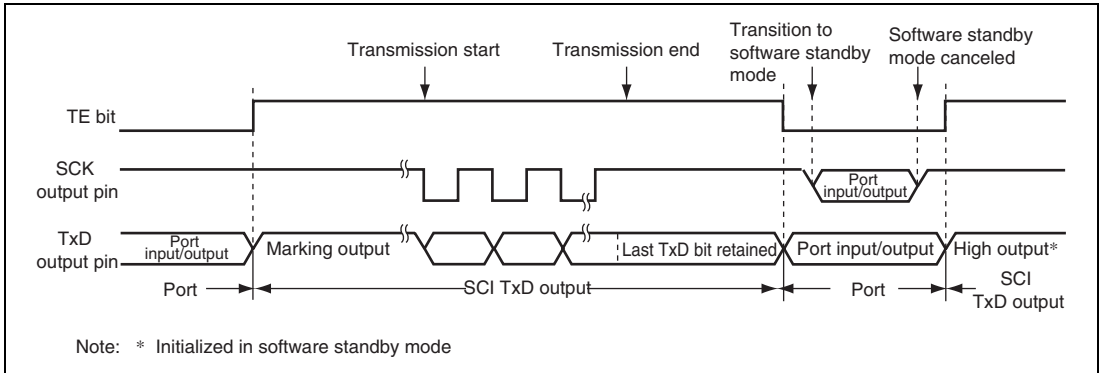
Figure 19.41 Port Pin States during Software Standby Mode Transition (Internal Clock, Clock Synchronous Transmission)
