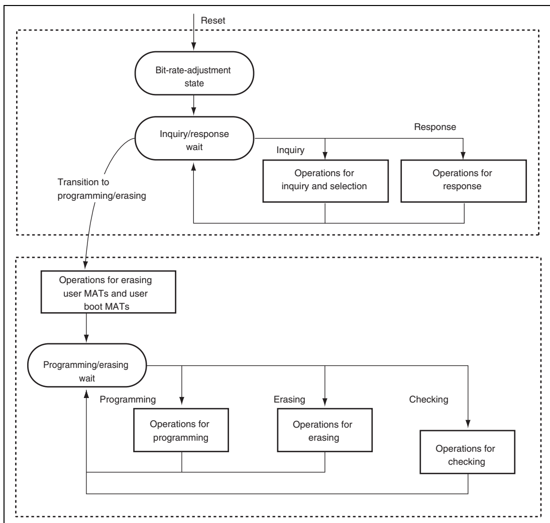
Figure 24.21 Boot Program States
