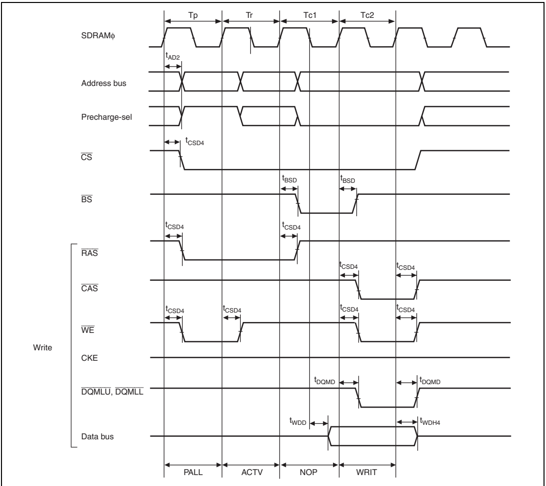
Figure 29.30 Synchronous DRAM Basic Write Access Timing (CAS Latency 2)*
