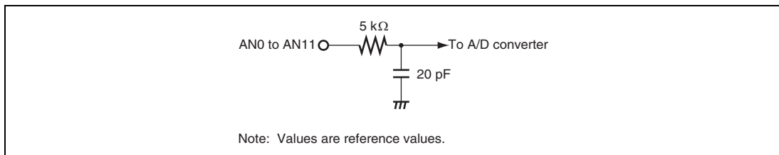
Figure 21.15 Analog Input Pin Equivalent Circuit
