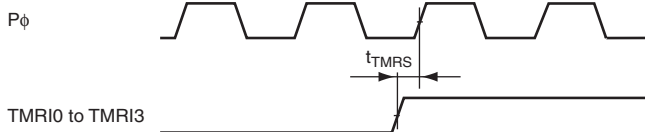
Figure 29.47 8-Bit Timer Reset Input Timing
