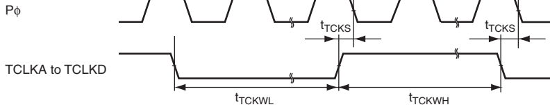
Figure 29.44 TPU Clock Input Timing
