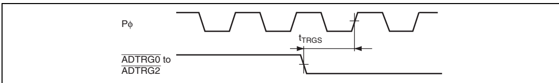
Figure 29.52 A/D Converter External Trigger Input Timing
