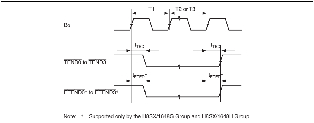
Figure 29.38 Timing of \overline{\text{TEND}} and \overline{\text{ETEND}}^* input (for the DMAC and EXDMAC*)
