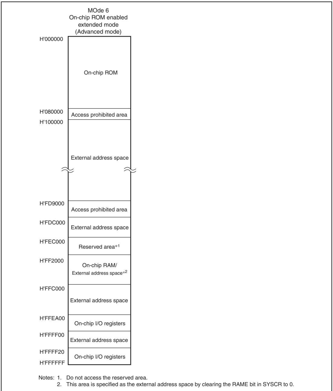
Figure 3.2 Address Map in Each Operating Mode of H8SX/1644, 1644A, 1644L, 1644G, and 1644H (2)
