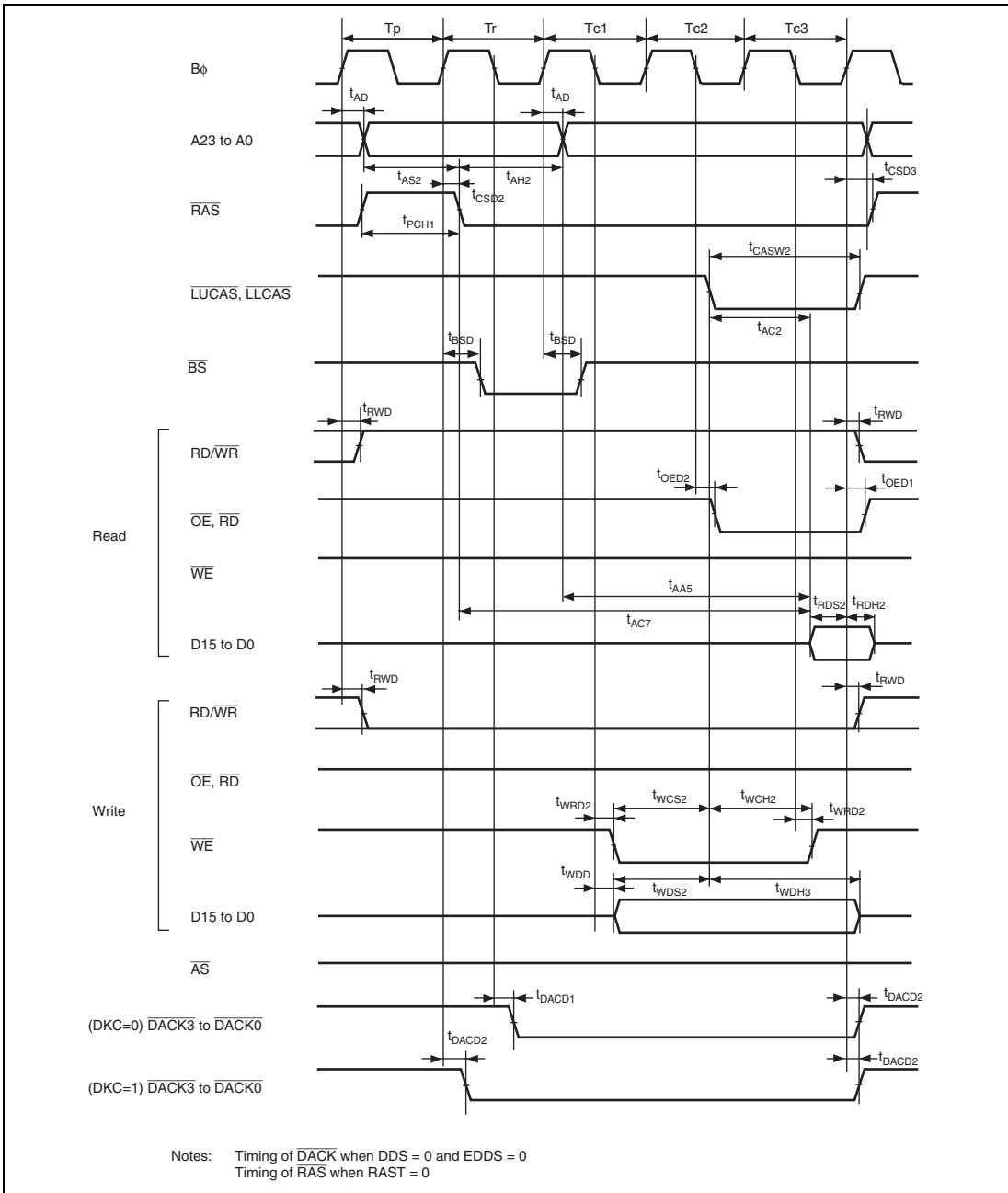
Figure 29.22 DRAM Access Timing / Three-State Access (When RAST=1)*
