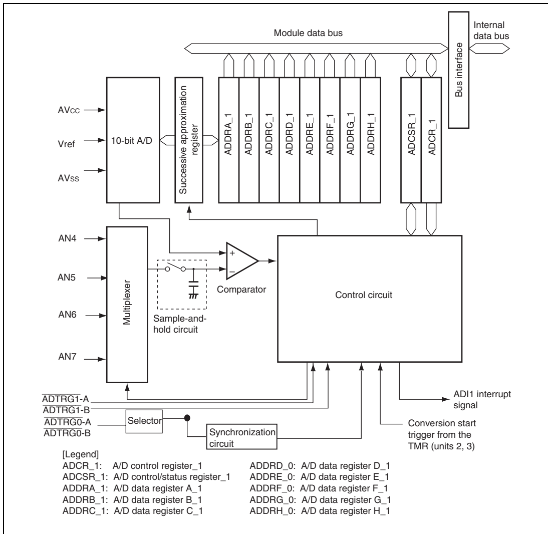
Figure 21.2 Block Diagram of A/D Converter Unit 1 (AD_1)
