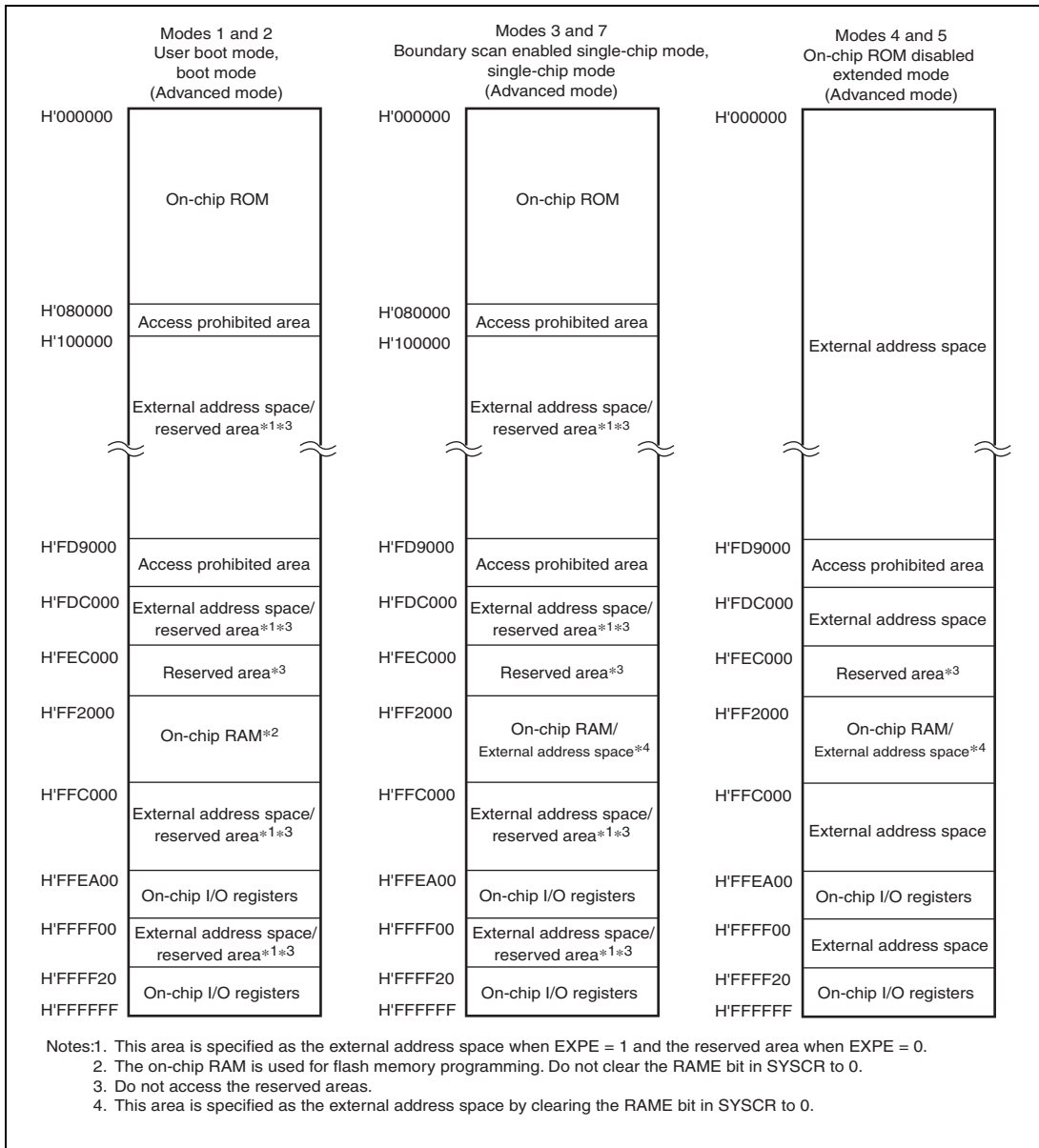
Figure 3.2 Address Map in Each Operating Mode of H8SX/1644, 1644A, 1644L, 1644G, and 1644H (1)
