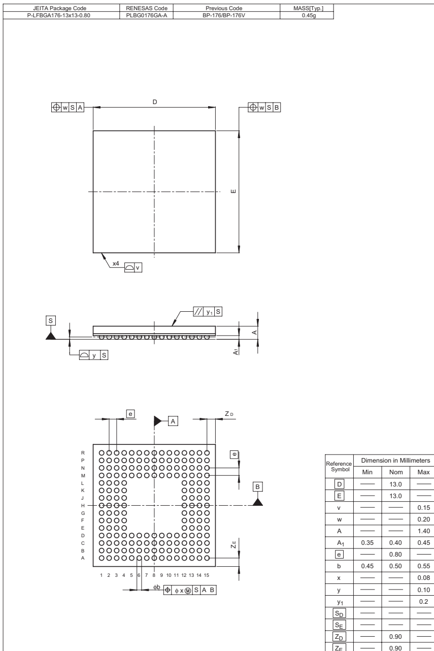
Figure C.2 Package Dimensions (BP-176V)
