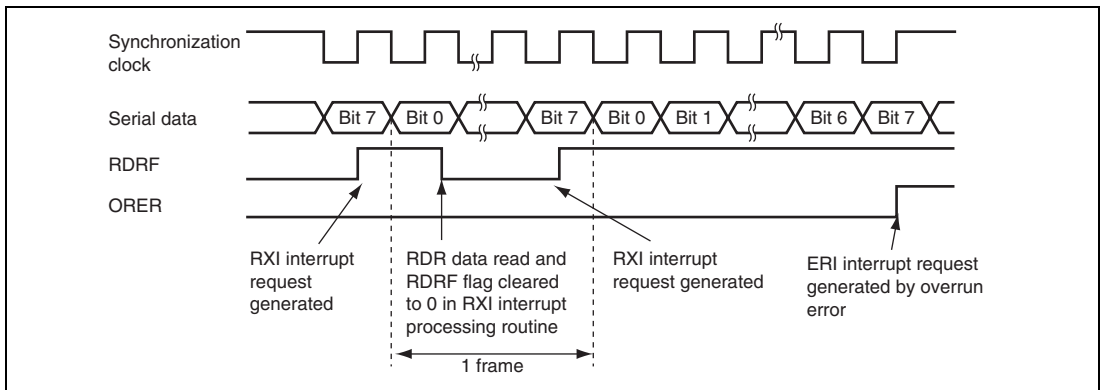
Figure 19.21 Example of Operation for Reception in Clock Synchronous Mode
