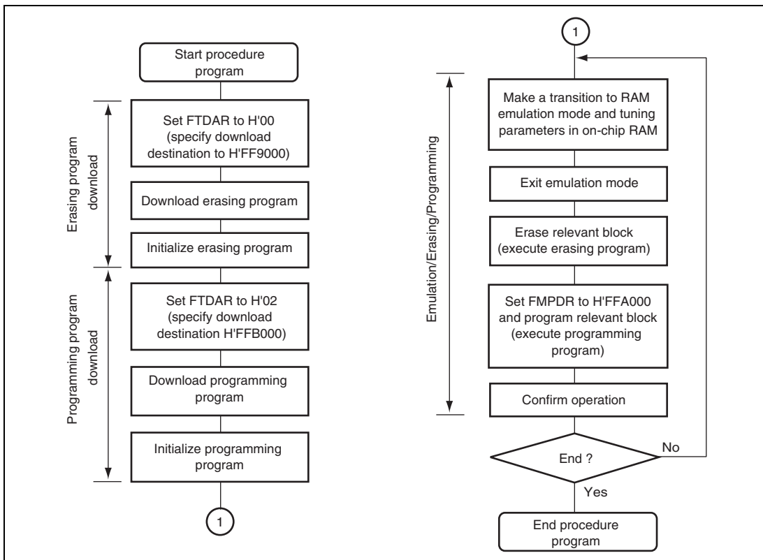
Figure 24.13 Repeating Procedure of Erasing, Programming, and RAM Emulation in User Program Mode
