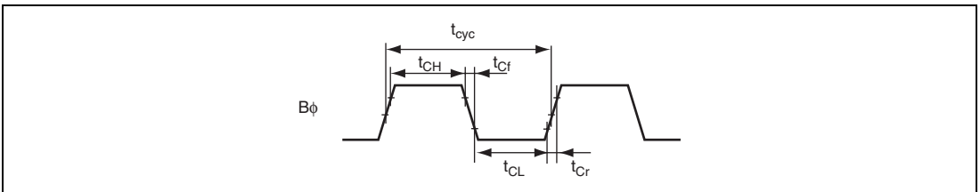
Figure 29.2 External Bus Clock Timing
