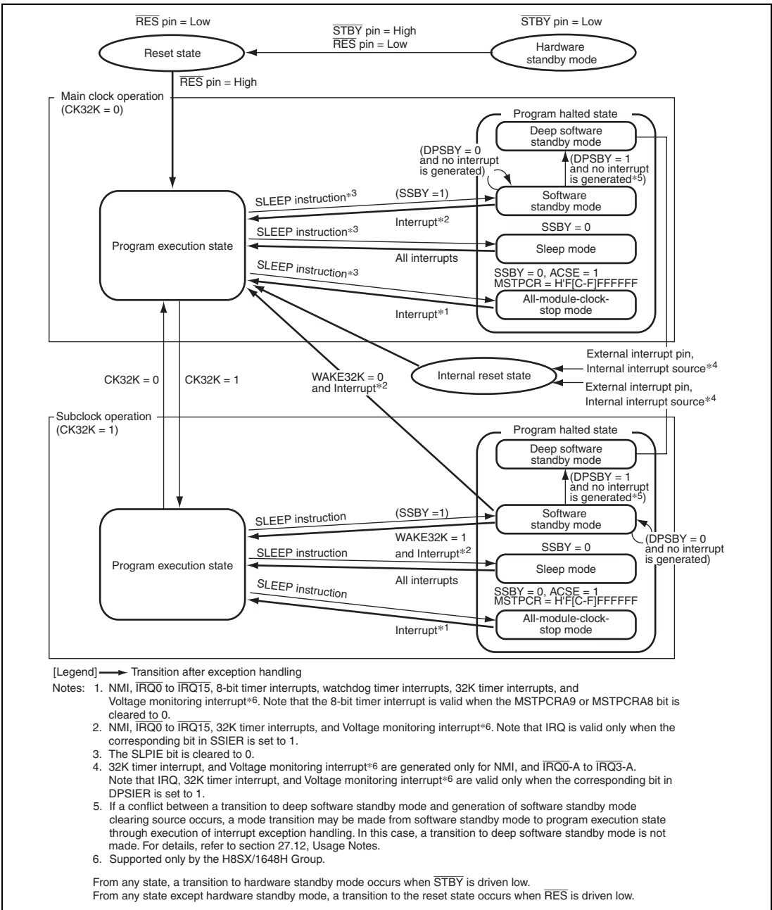
Figure 27.1 (2) Mode Transitions (H8SX/1648G Group and H8SX/1648H Group)
