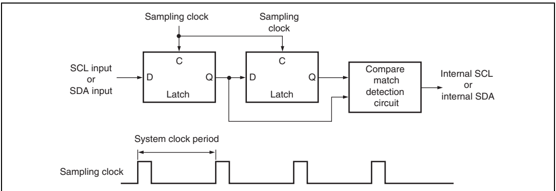
Figure 20.13 Block Diagram of Noise Canceller
