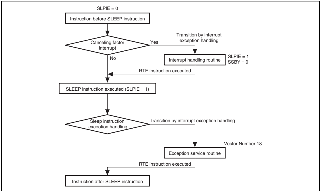
Figure 27.12 When Canceling Factor Interrupt is Generated before SLEEP Instruction Execution (Sleep Instruction Exception Handling Initiated)
