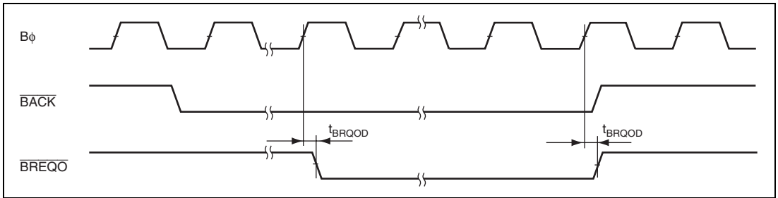
Figure 29.36 External Bus Request Output Timing
