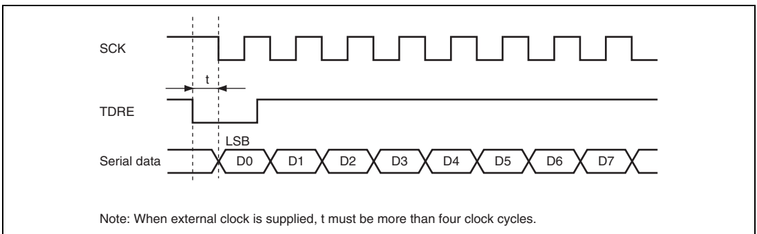
Figure 19.38 Sample Transmission using DTC in Clock Synchronous Mode
