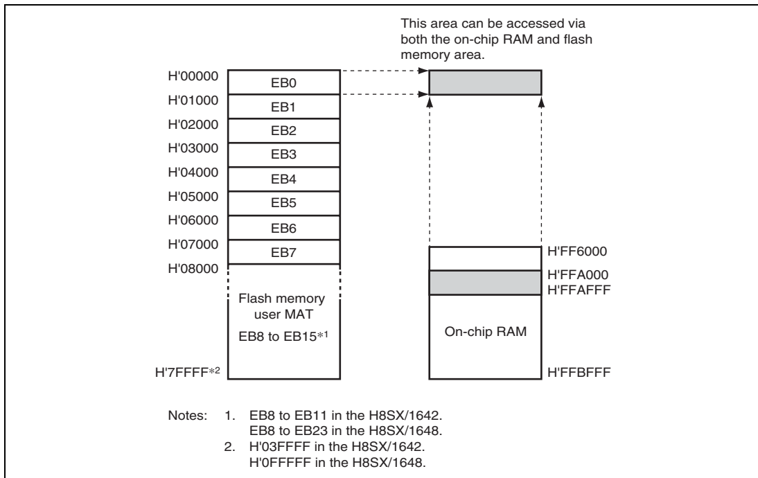
Figure 24.18 Address Map of Overlaid RAM Area (H8SX/1644)
