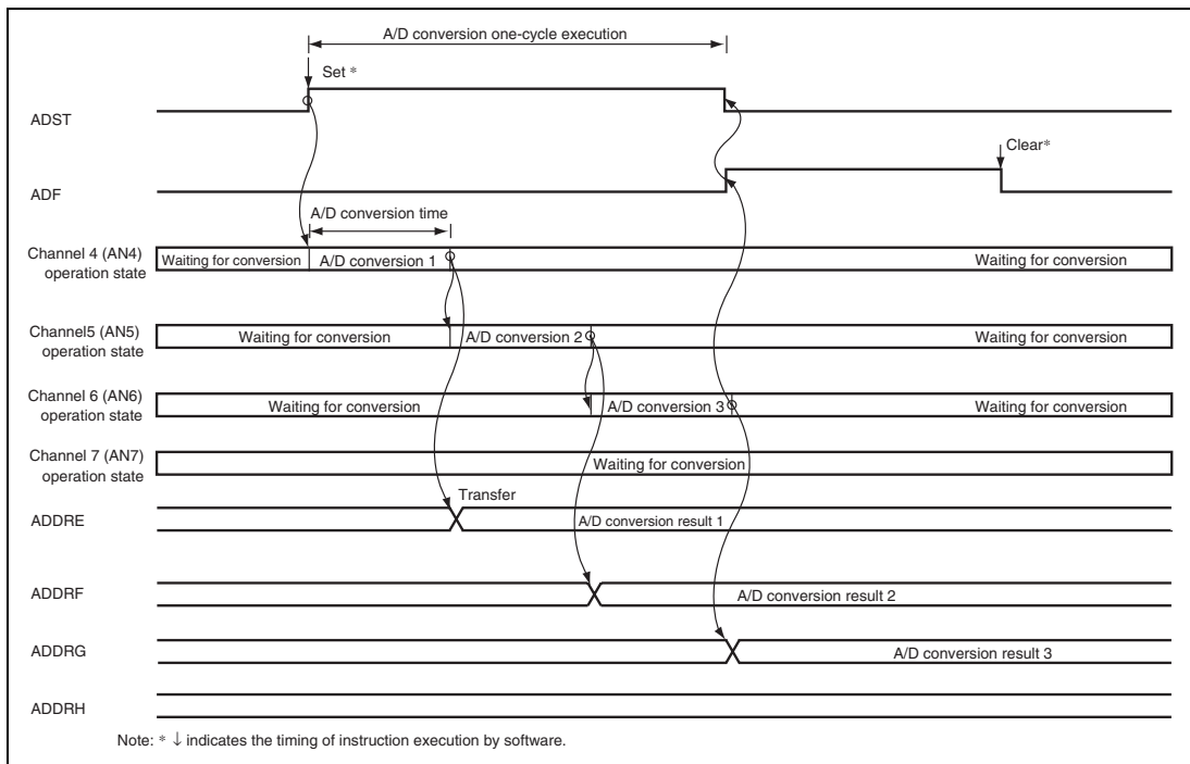
Figure 21.6 Example of A/D Conversion (One-Cycle Scan Mode, Three Channels (AN4 to AN6) Selected)
