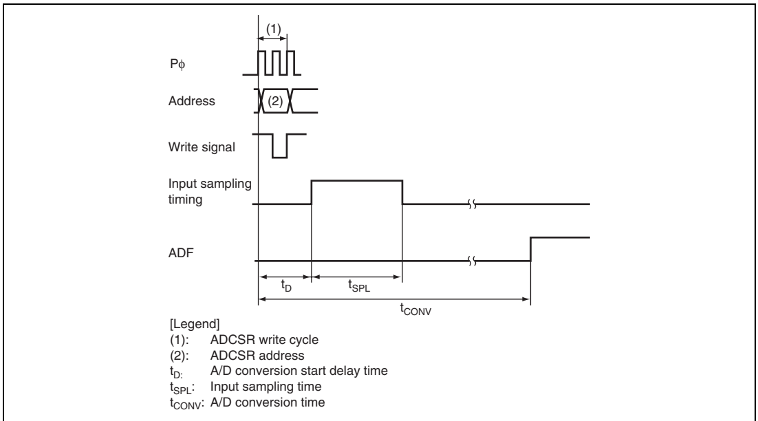
Figure 21.7 A/D Conversion Timing
