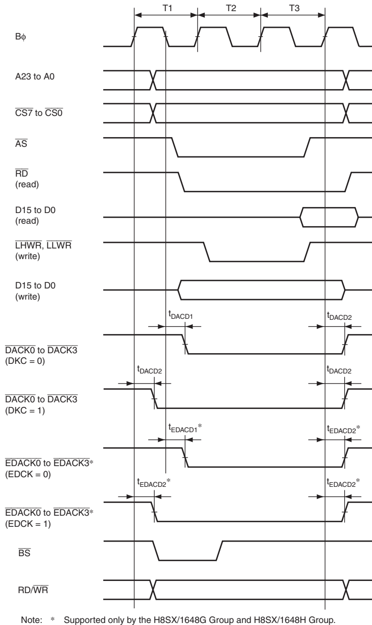
Figure 29.40 Single Address Transfer Timing for the DMAC and EXDMAC* (Three-State Access)
