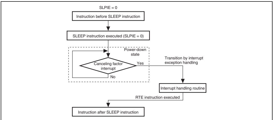
Figure 27.10 When Canceling Factor Interrupt is Generated after SLEEP Instruction Execution
