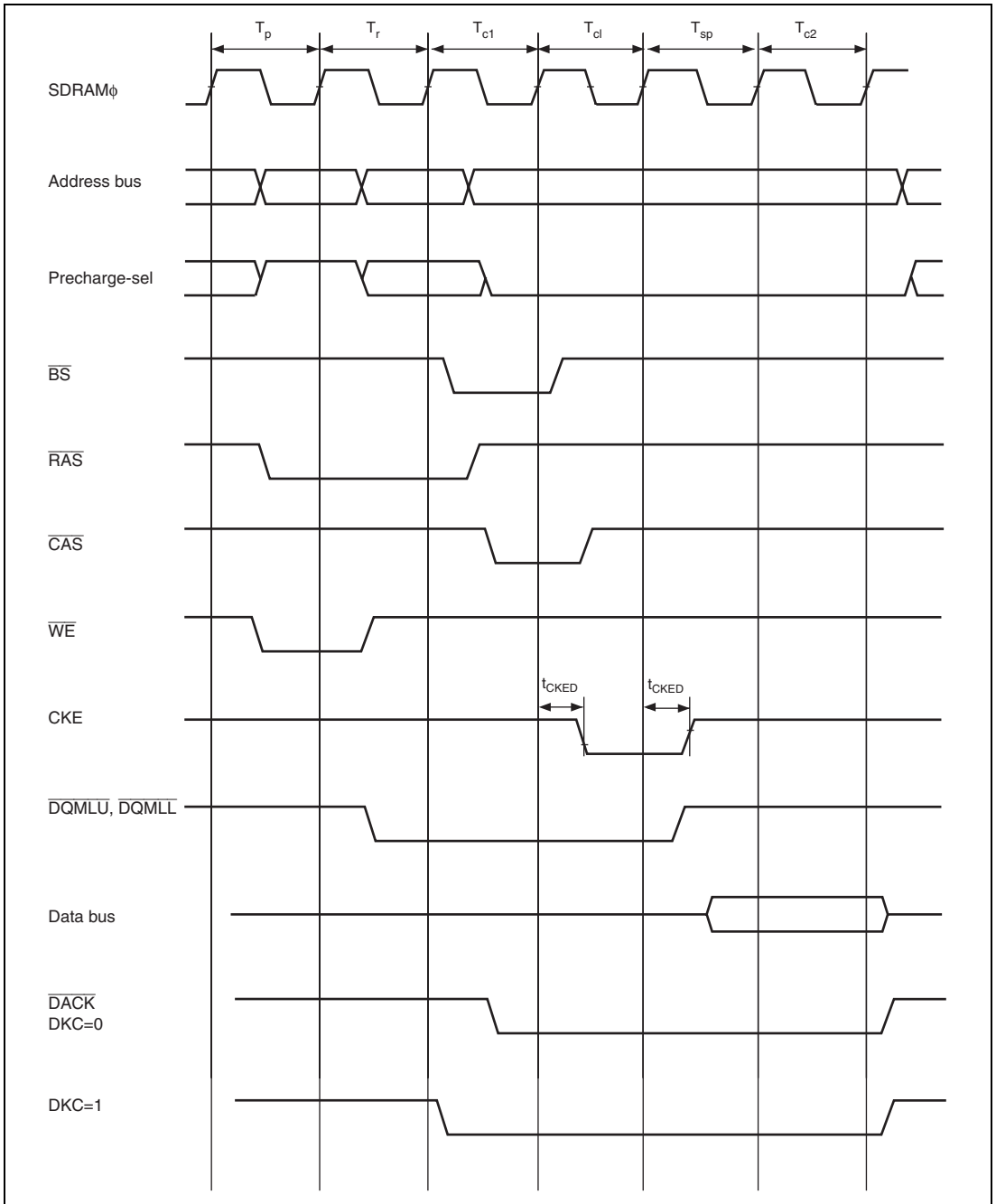
Figure 29.31 Extended Read Data Cycle (CAS Latency 2)*
