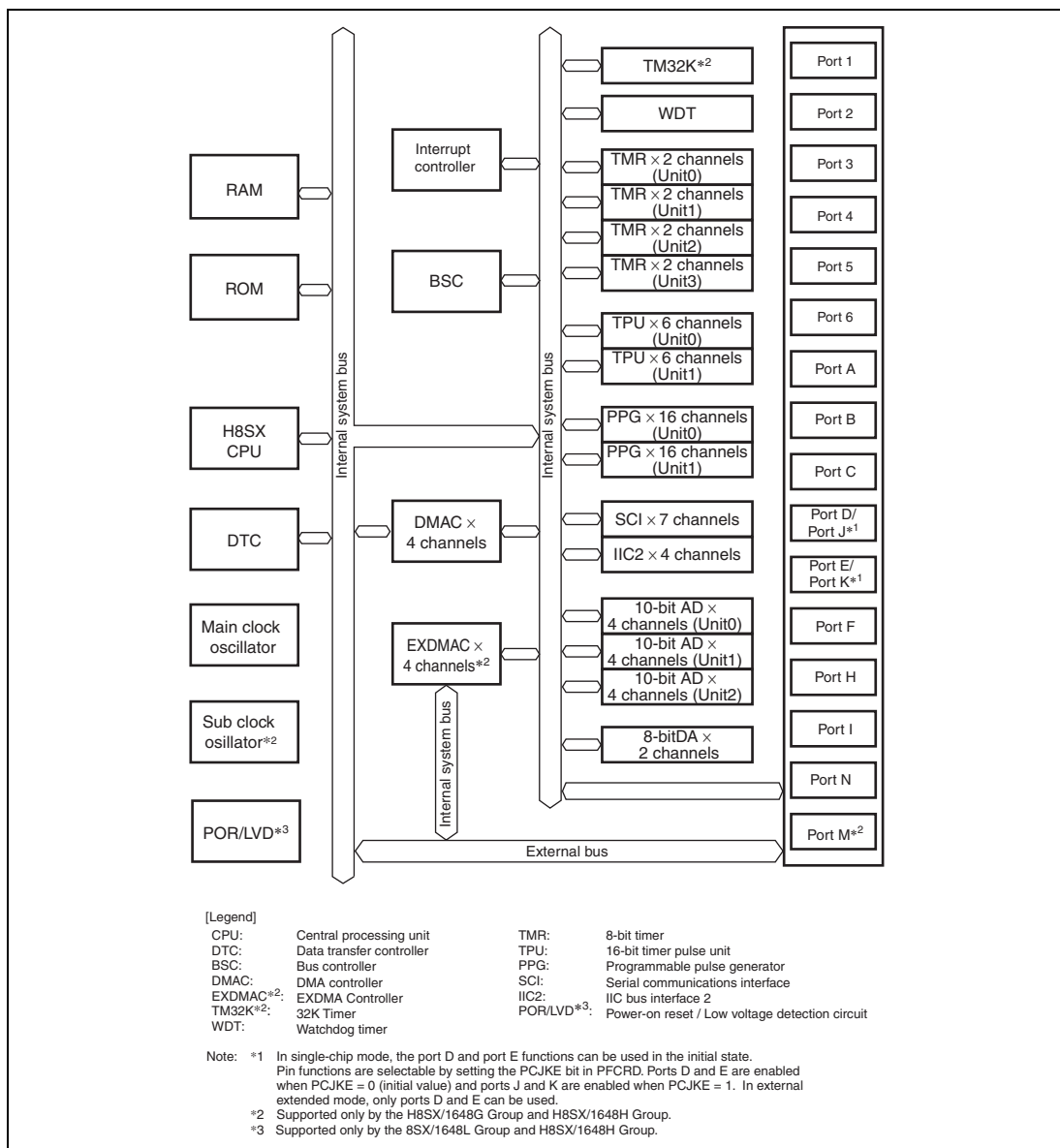
Figure 1.2 Block Diagram
