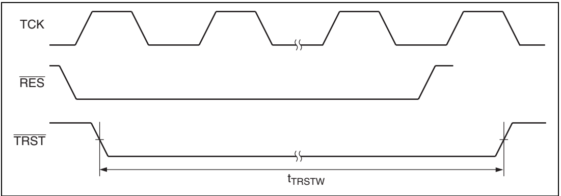
Figure 29.55 Boundary Scan \overline{TRST} Timing
