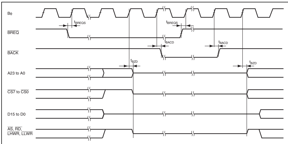
Figure 29.35 External Bus Release Timing
