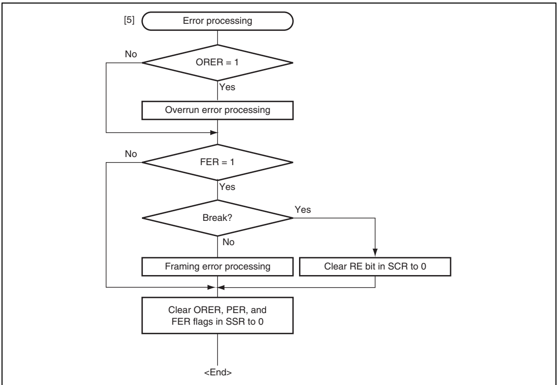
Figure 19.16 Sample Multiprocessor Serial Reception Flowchart (2)
