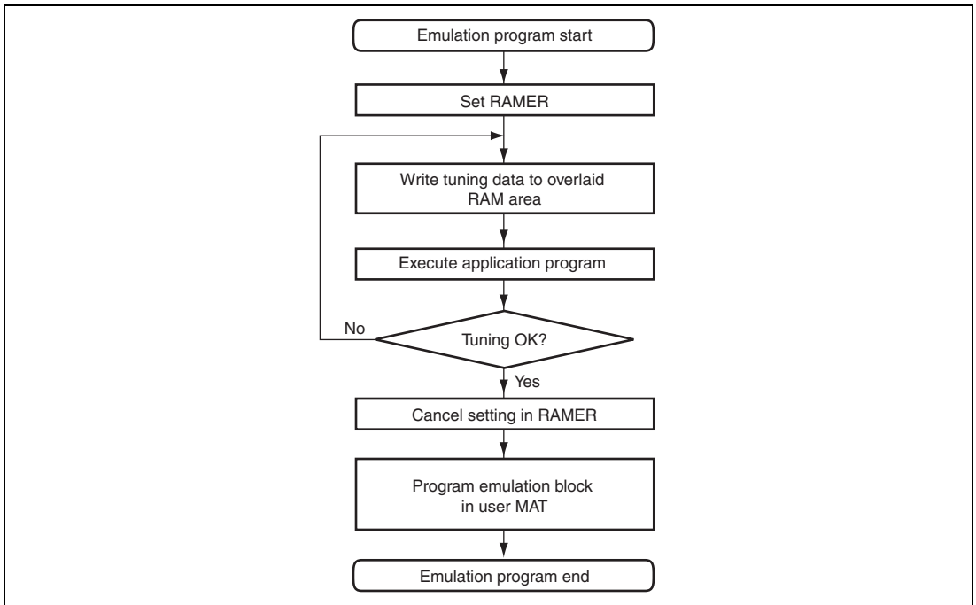
Figure 24.17 RAM Emulation Flow
