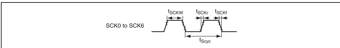
Figure 29.50 SCK Clock Input Timing
