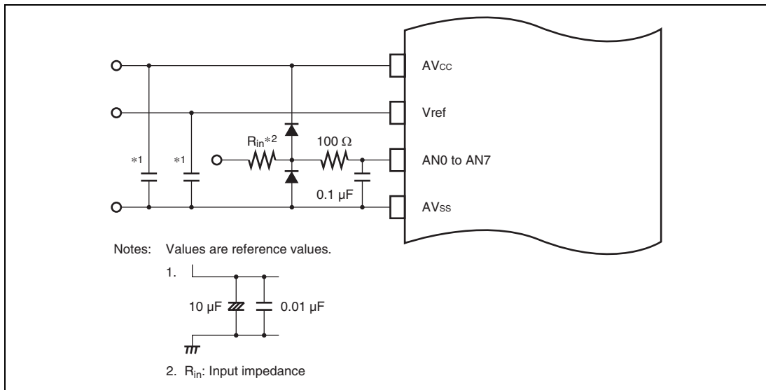
Figure 21.14 Example of Analog Input Protection Circuit
