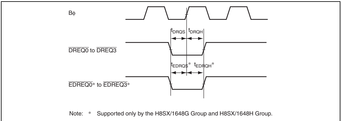
Figure 29.37 Timing of \overline{\text{DREQ}} and \overline{\text{EDREQ}}^* input (for the DMAC and EXDMAC*)
