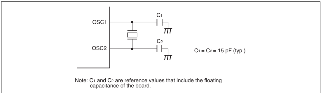
Figure 26.6 Connection Example of 32.768-kHz Crystal Resonator
