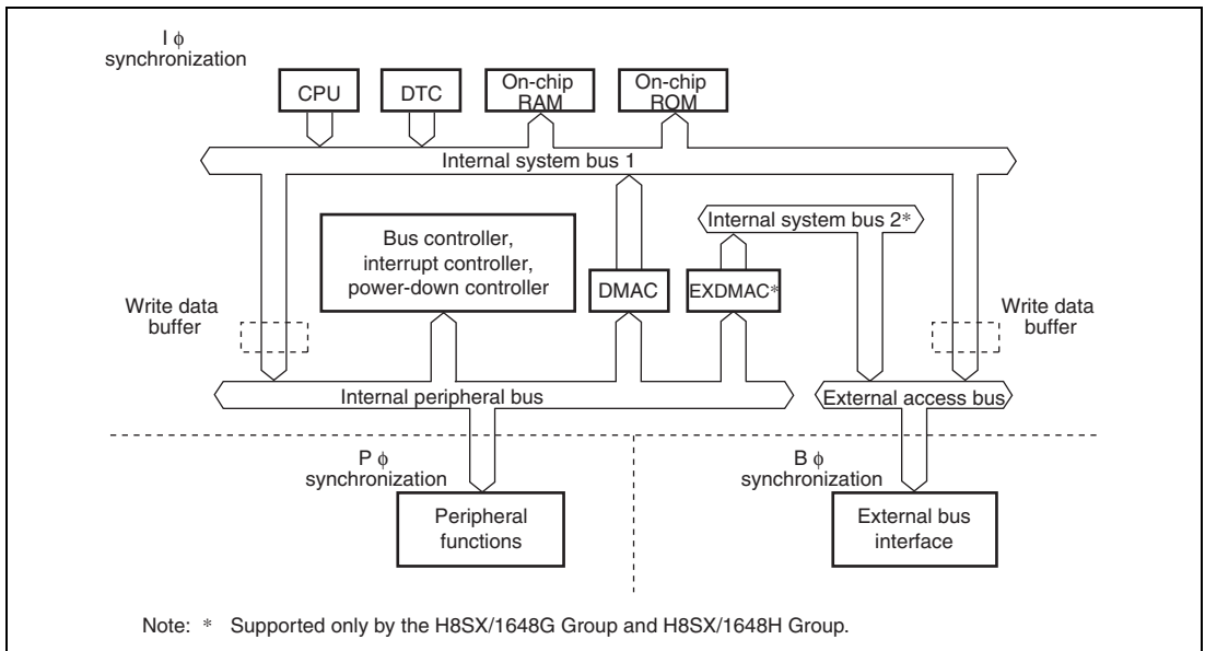
Figure 9.5 Internal Bus Configuration
