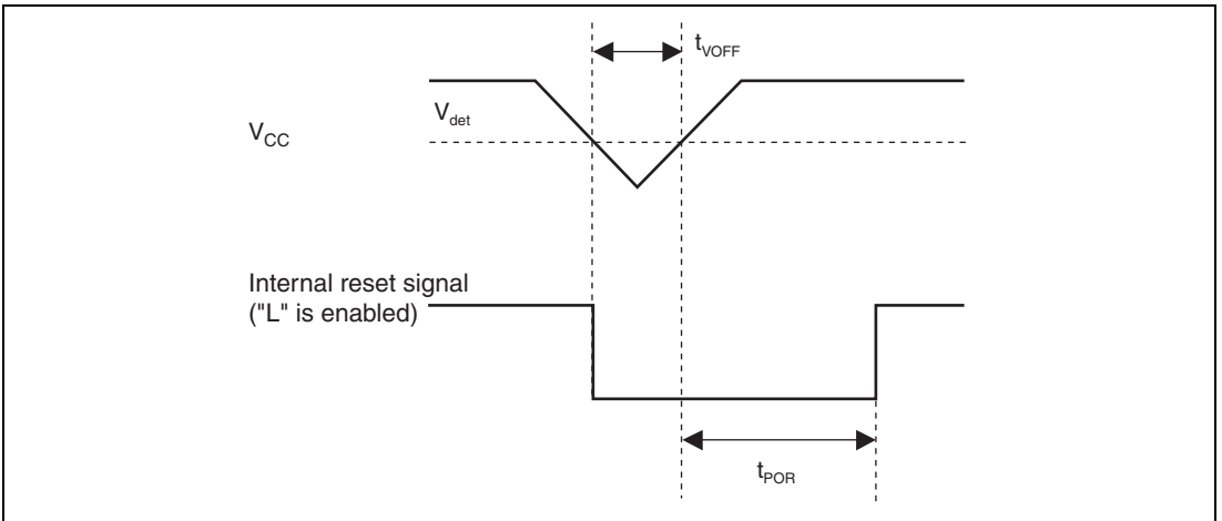
Figure 29.58 Voltage Detection Circuit Timing
