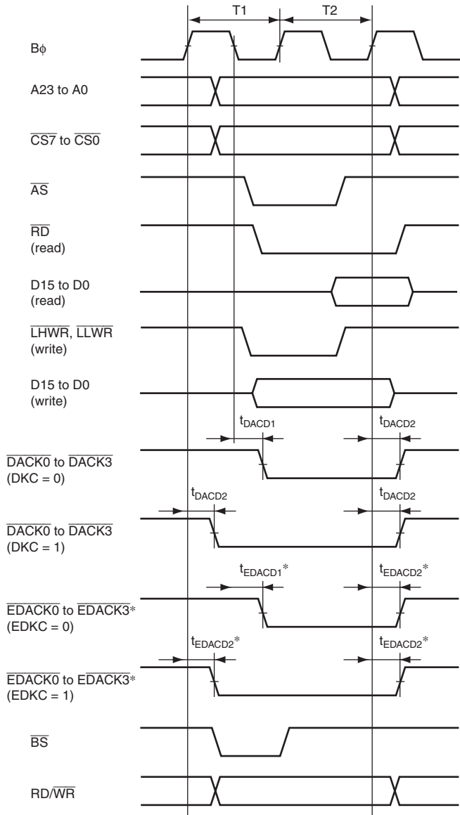
Figure 29.39 Single Address Transfer Timing for the DMAC and EXDMAC* (Two-State Access)
