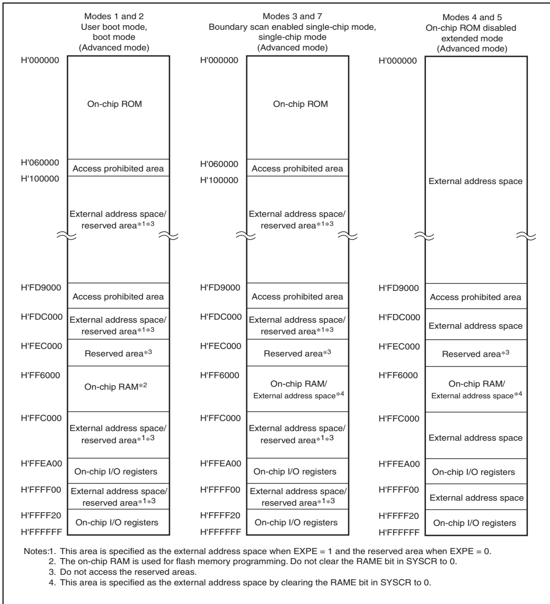
Figure 3.3 Address Map in Each Operating Mode of H8SX/1642, 1642A, 1642L, 1642G, and 1642H (1)
