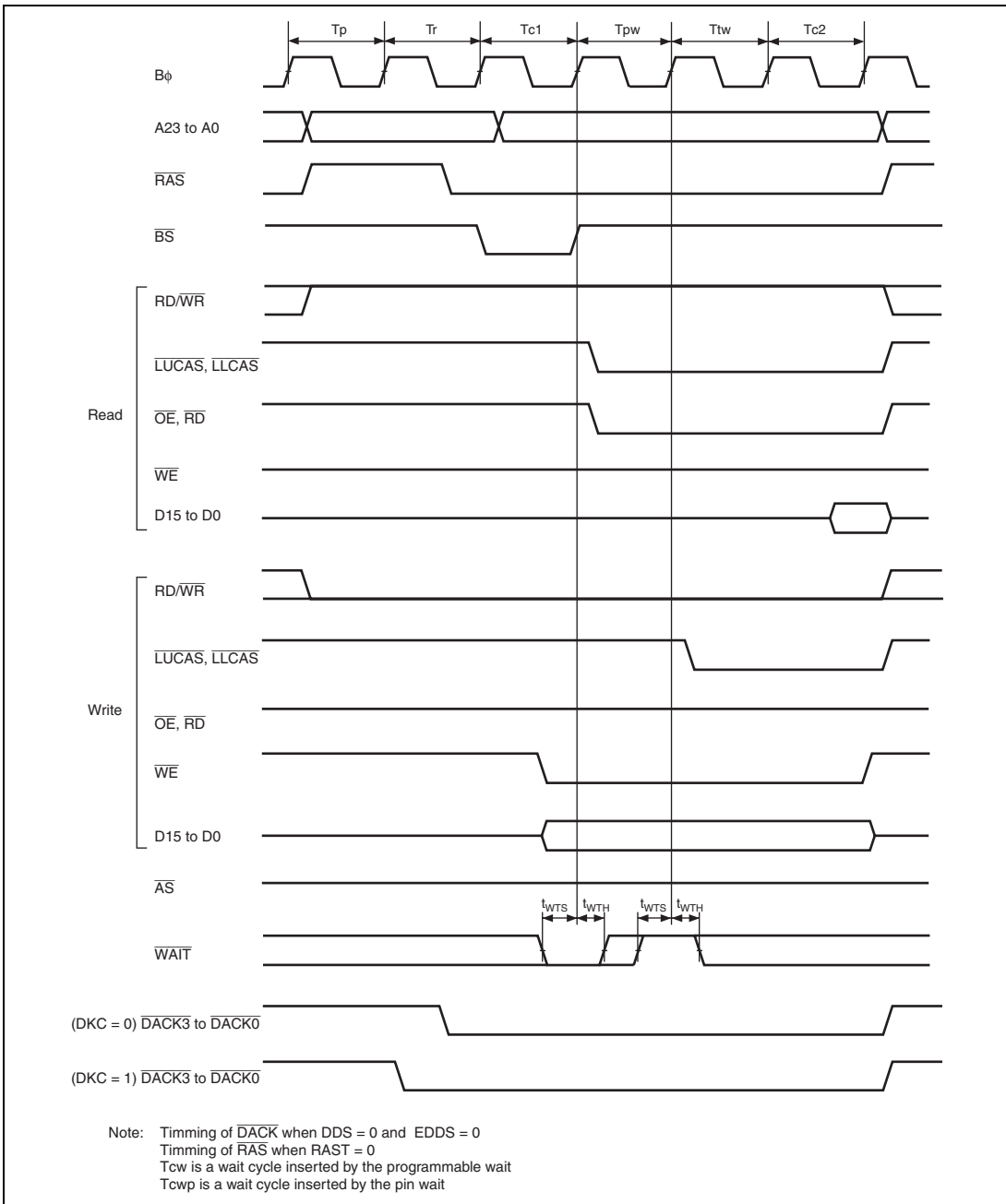
Figure 29.20 DRAM Access Timing / Two-State Access, One Wait*
