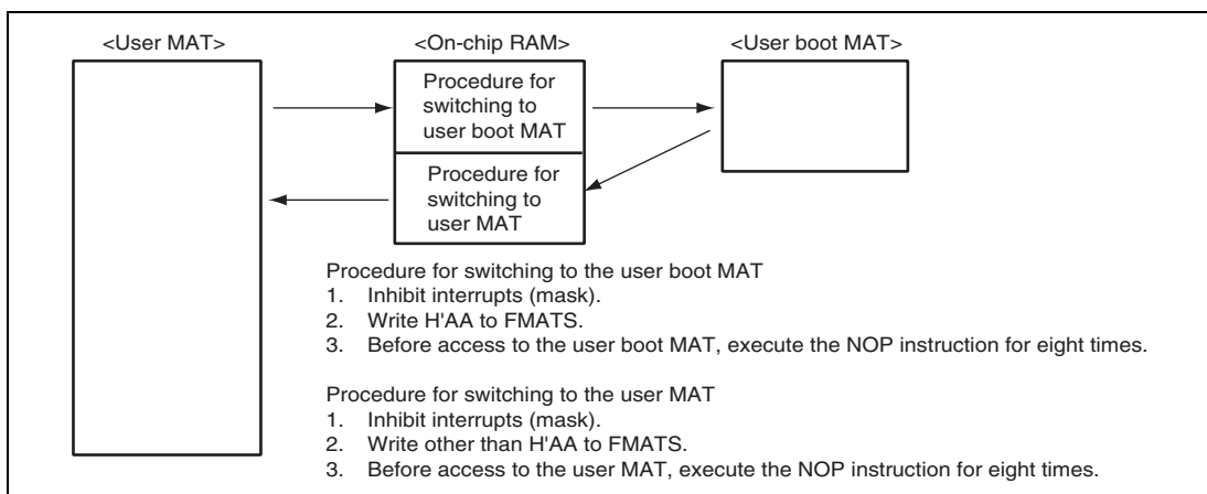
Figure 24.20 Switching between User MAT and User Boot MAT
