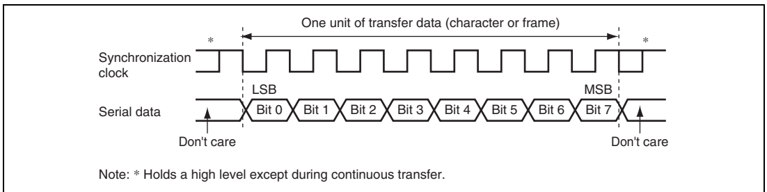
Figure 19.17 Data Format in Clock Synchronous Communication (LSB-First)
