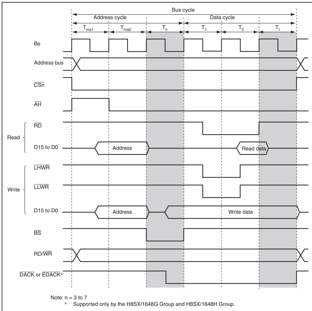
Figure 9.35 Chip Select ( \overline{\text{CS}} ) Assertion Period Extension Timing in Data Cycle
