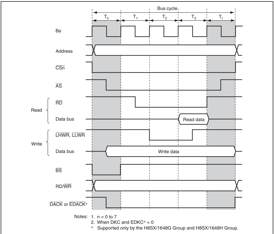
Figure 9.23 Example of Timing when Chip Select Assertion Period is Extended
