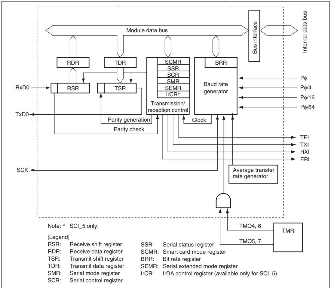
Figure 19.2 Block Diagram of SCI_5 and SCI_6
