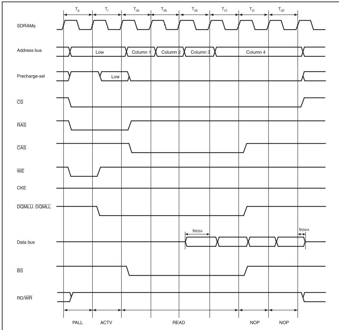
Figure 29.32 Synchronous DRAM Cluster Transfer Access Timing (Read)*
