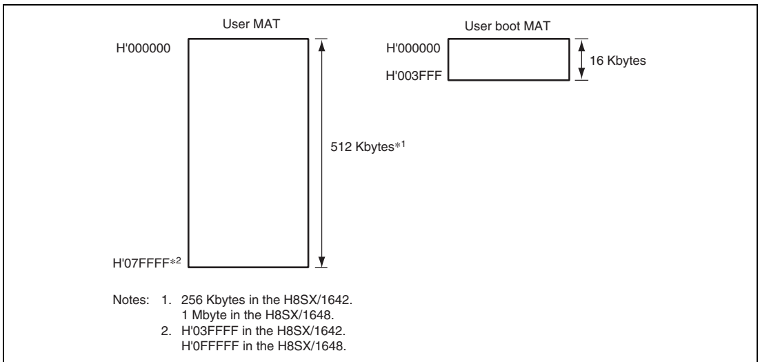
Figure 24.3 Memory MAT Configuration (H8SX/1644)
