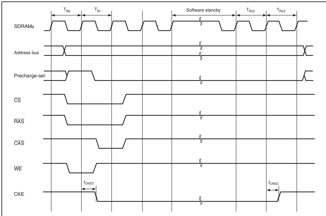
Figure 29.34 Synchronous DRAM Self-Refresh Timing*
