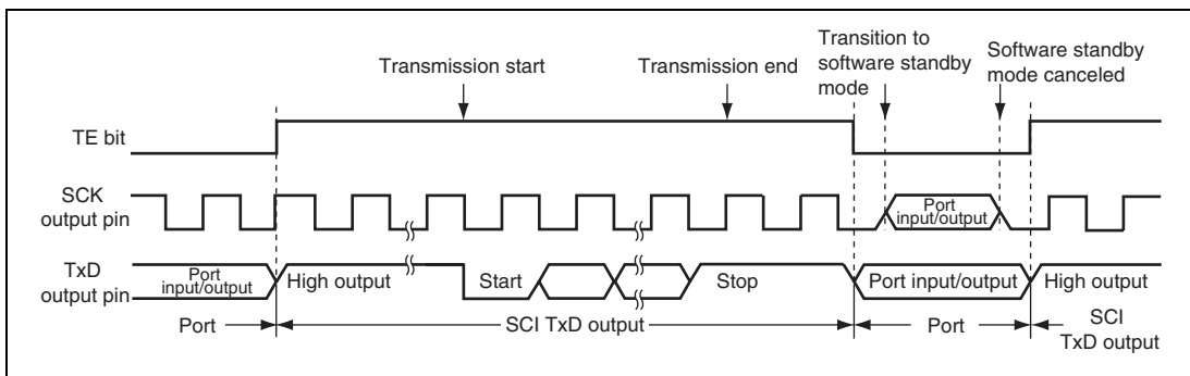
Figure 19.40 Port Pin States during Software Standby Mode Transition (Internal Clock, Asynchronous Transmission)
