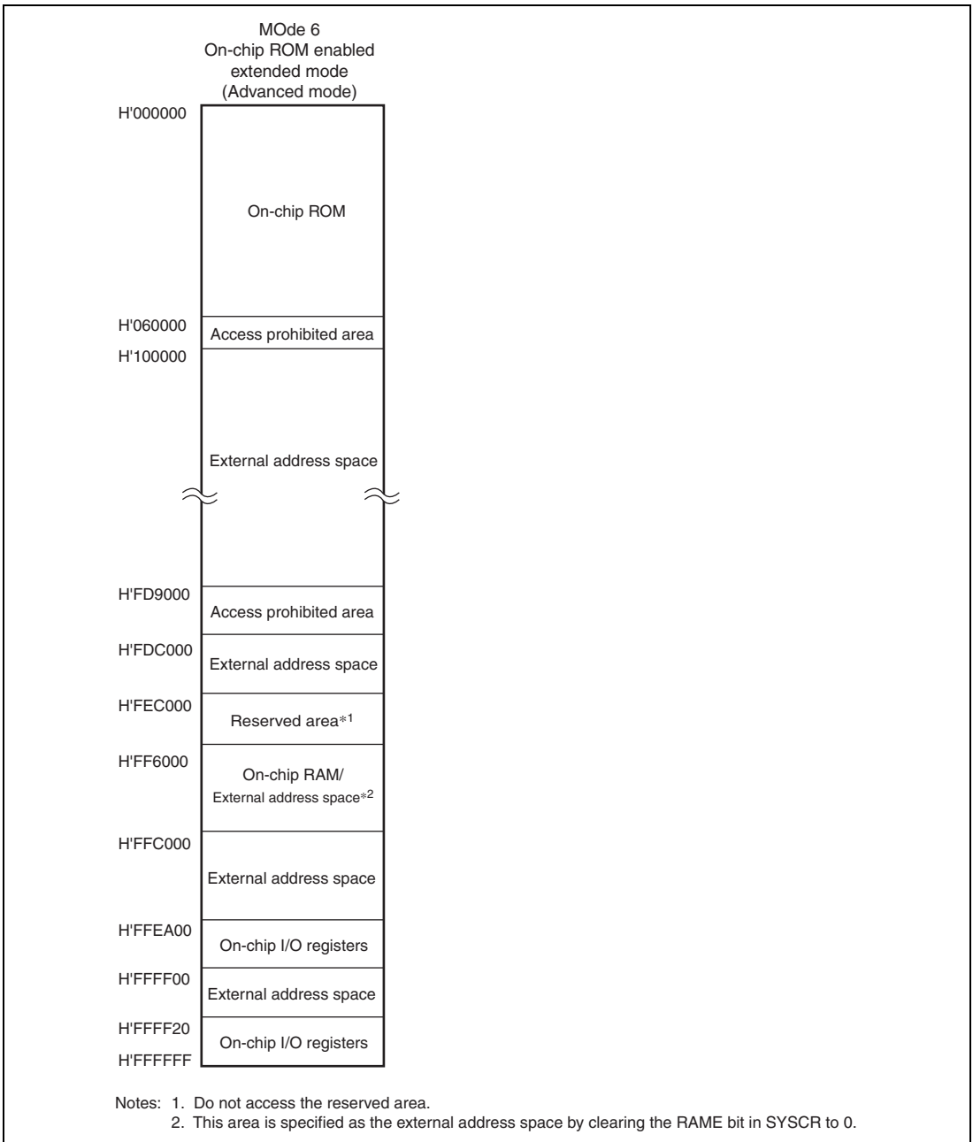
Figure 3.3 Address Map in Each Operating Mode of H8SX/1642, 1642A, 1642L, 1642G, and 1642H (2)
