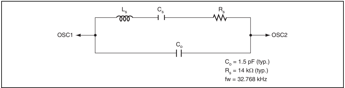
Figure 26.7 Equivalent Circuit for 32.768-kHz Crystal Resonator
