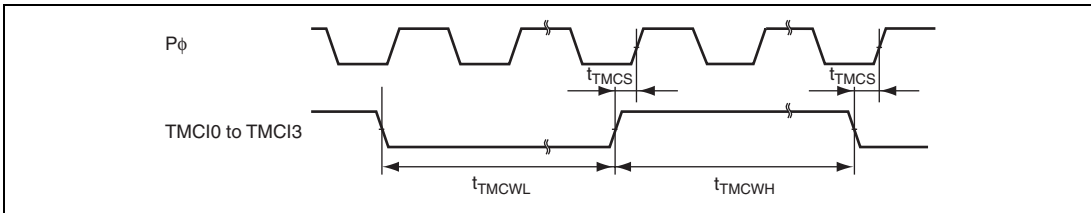
Figure 29.48 8-Bit Timer Clock Input Timing
