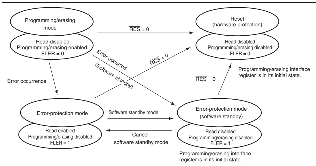
Figure 24.16 Transitions to Error Protection State
