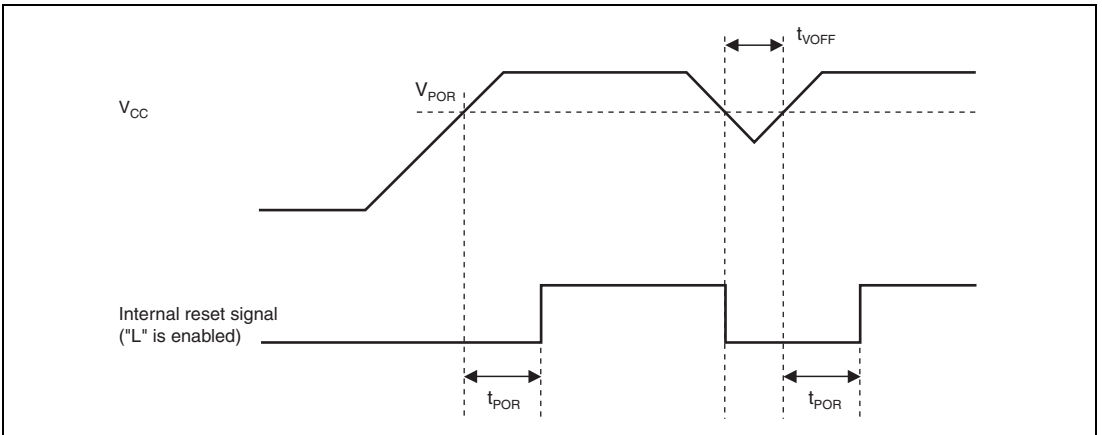
Figure 29.57 Power-On Reset Timing
