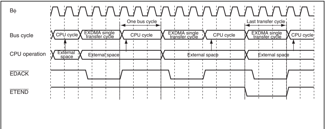
Figure 11.40 Auto-Request/Normal Transfer Mode/Cycle Steal Mode (CPU Cycles/Single Address Mode)
