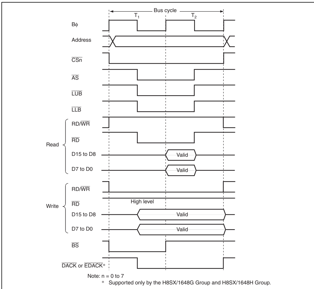
Figure 9.25 16-Bit 2-State Access Space Bus Timing
