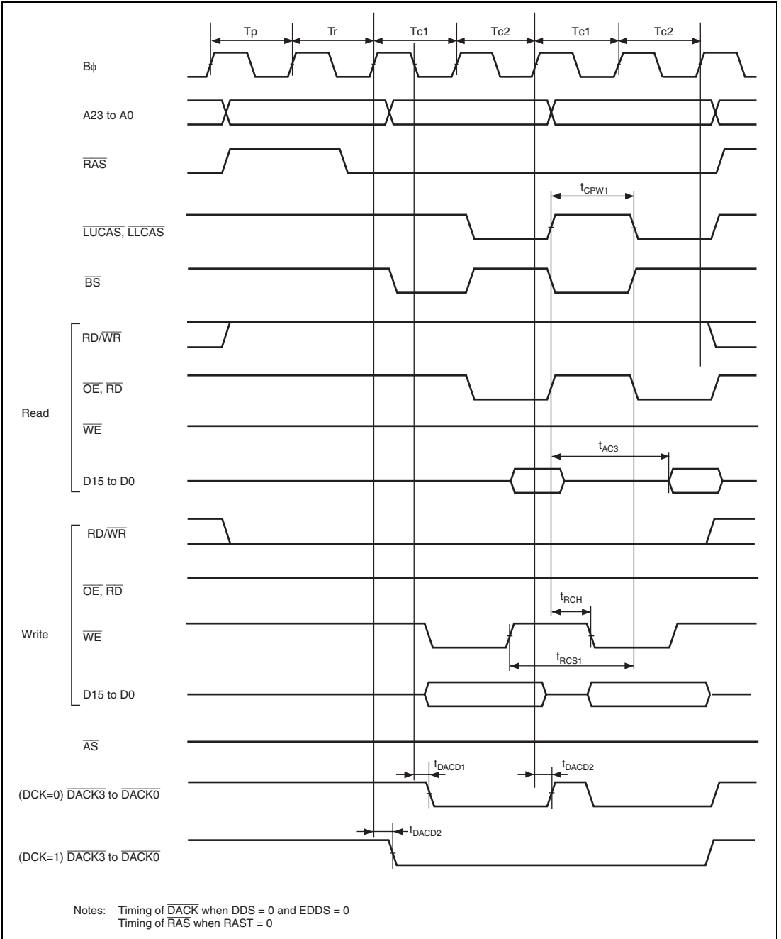
Figure 29.21 DRAM Access Timing / Two-State Burst Access*
