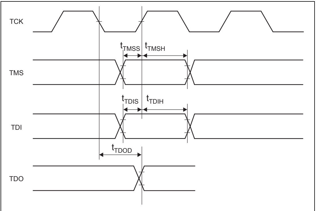
Figure 29.56 Boundary Scan Input/Output Timing
