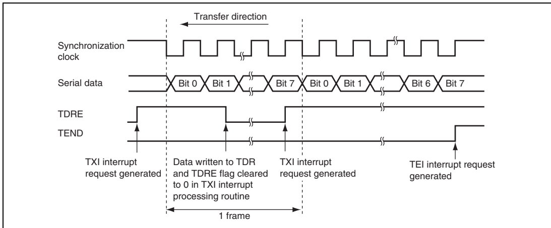
Figure 19.19 Example of Operation for Transmission in Clock Synchronous Mode
