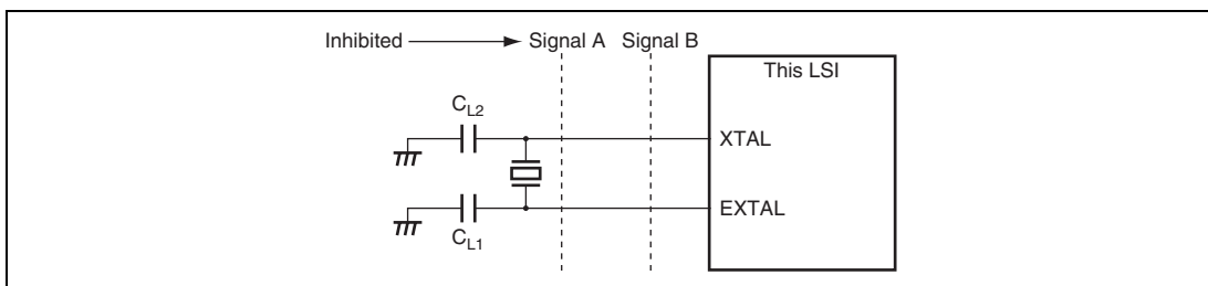
Figure 26.10 Note on Board Design for Oscillation Circuit
