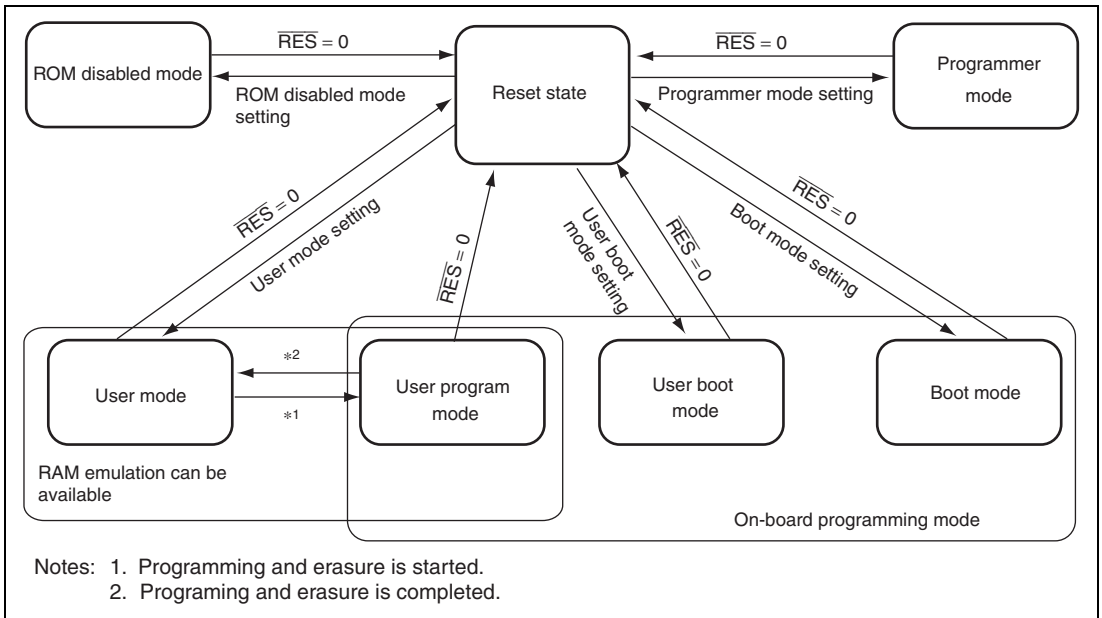
Figure 24.2 Mode Transition of Flash Memory
