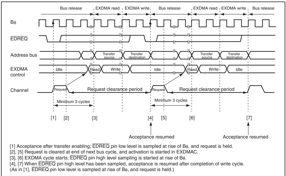
Figure 11.29 Example of Normal Transfer Mode Transfer Activated by \overline{\text{EDREQ}} Pin Falling Edge
