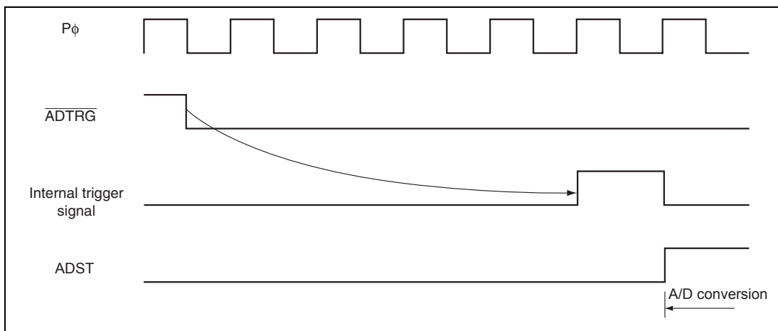
Figure 21.9 External Trigger Input Timing when Multiple Units Start Simultaneously (TRSG1, TRGS0, and EXTRGS = B'111)
