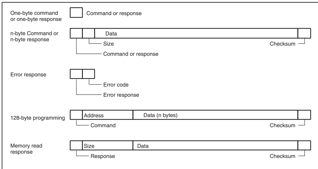
Figure 24.23 Communication Protocol Format
