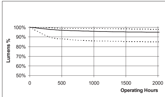
Figure 4. Lumen Maintenance.
