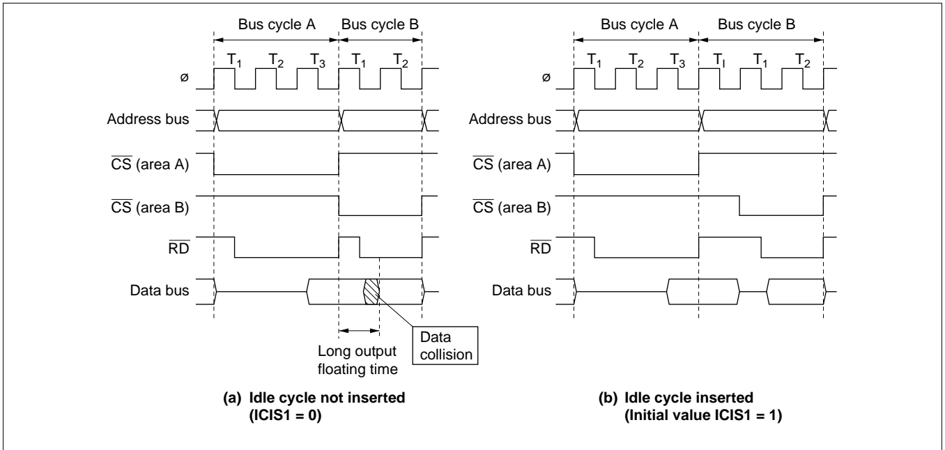
Figure 6-31 Example of Idle Cycle Operation (1)
