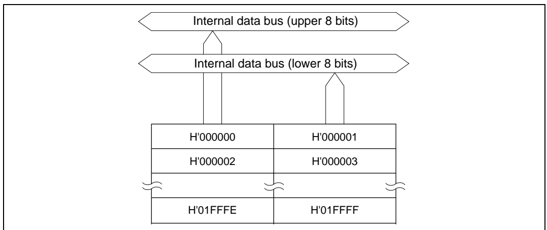
Figure 21.1 ROM Block Diagram (H8S/2138, H8S/2134)
