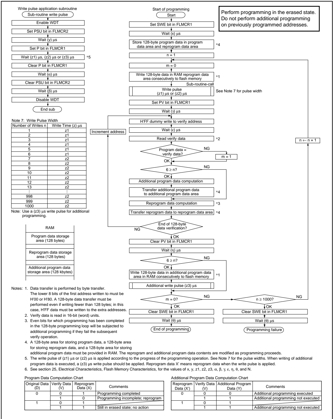
Figure 22.12 Program/Program-Verify Flowchart
