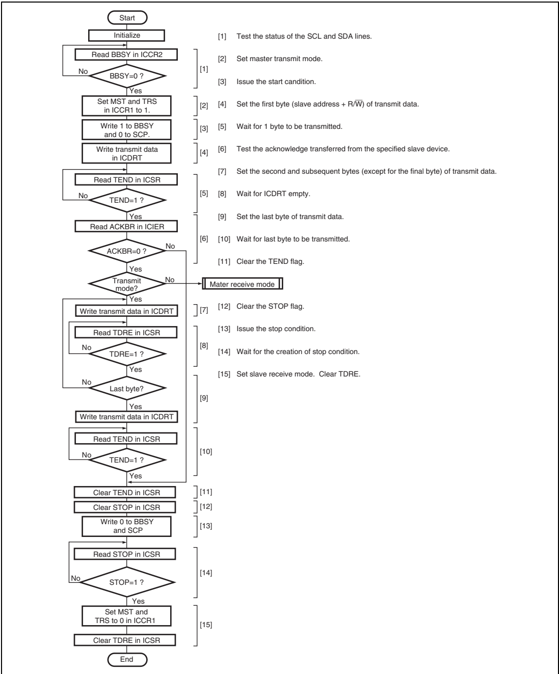
Figure 20.14 Sample Flowchart for Master Transmit Mode
