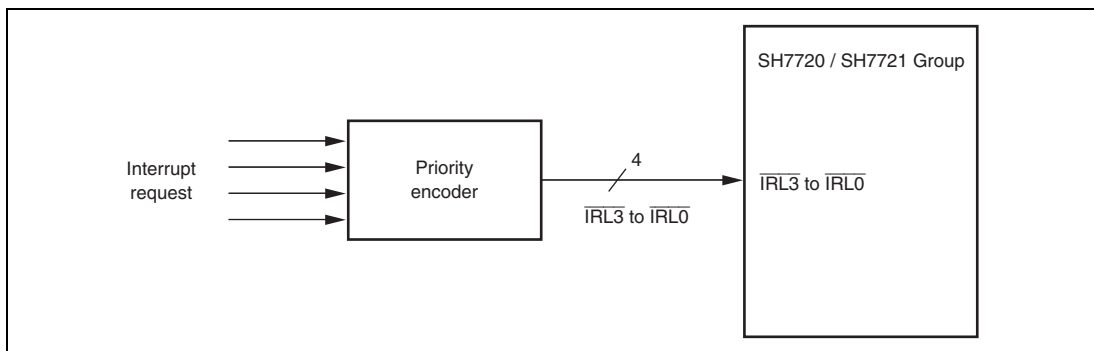
Figure 8.2 Example of IRL Interrupt Connection
