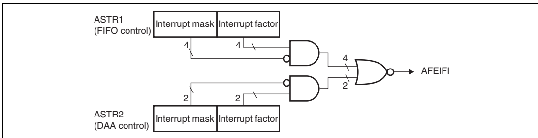
Figure 22.4 Interrupt Generator
