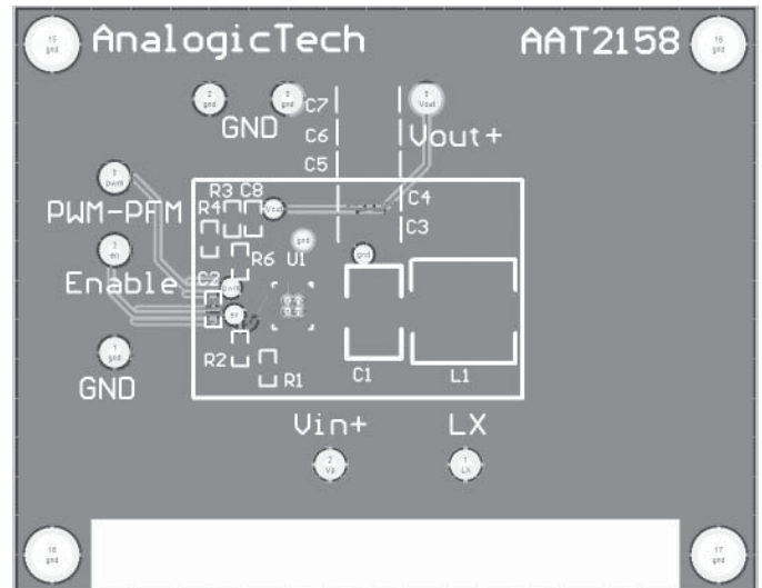
Figure 3: AAT2158 Evaluation Board Bottom Side Layout.
