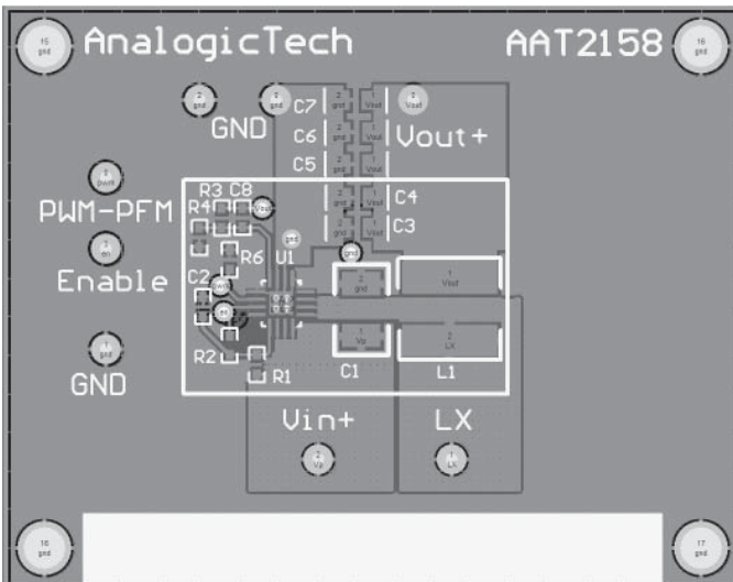
Figure 2: AAT2158 Evaluation Board Top Side Layout.
