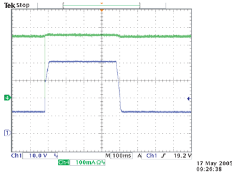
Fig. 6. LED current during step changes in the input voltage
