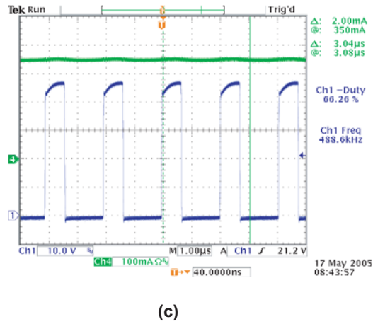
Fig. 4. Steady State Waveforms (a): 9V in; (b): 13.5V in; (c): 16V in
