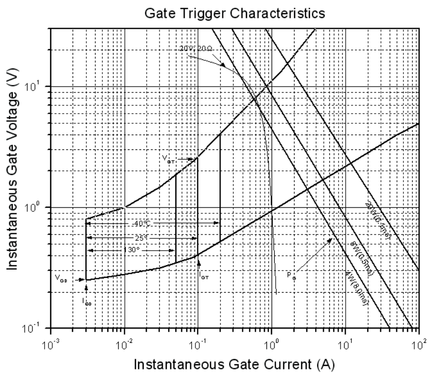
Fig. 7 - Gate Trigger Characteristics
