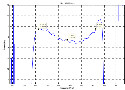
Phase Linearity(f0±5MHz)
