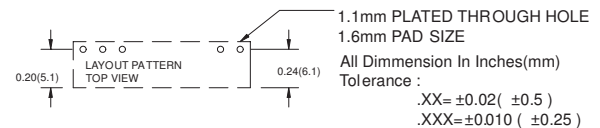
Figure 5. Recommended VPOL5A-12-SIP Footprint
