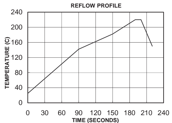
Figure 17 VPOL16A-12W-SMT Reflow Profile
