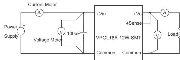
Figure 13. VPOL16A-12W-SMT Series Test Setup
