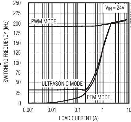
5V OUTPUT SWITCHING FREQUENCY vs. LOAD CURRENT (MAX8732)
