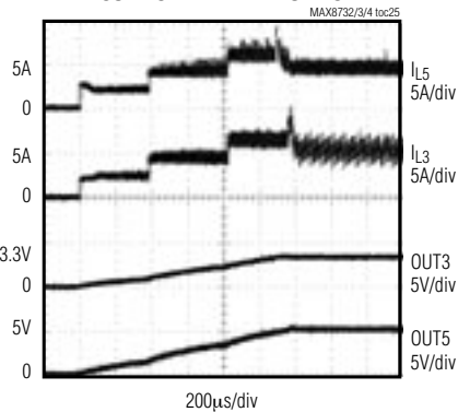
SOFT-START WAVEFORMS
