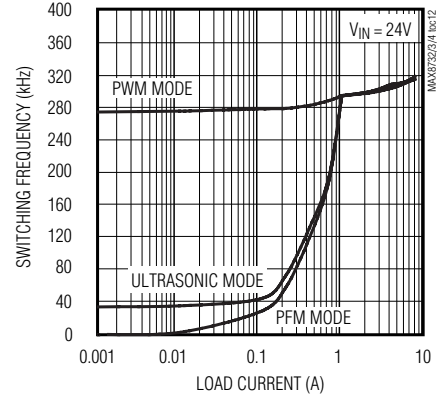
3.3V OUTPUT SWITCHING FREQUENCY vs. LOAD CURRENT (MAX8732)
