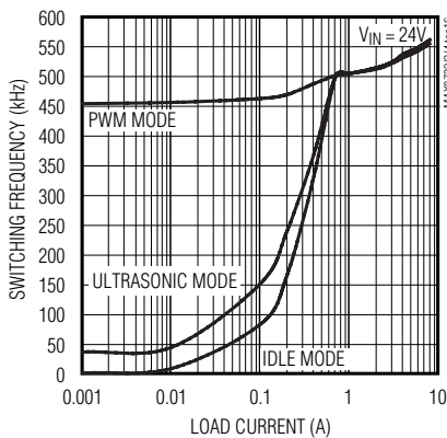
3.3V OUTPUT SWITCHING FREQUENCY vs. LOAD CURRENT (MAX8733)
