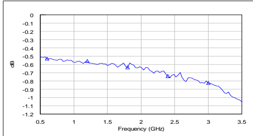
Insertion Loss
