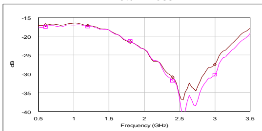
Return Loss
