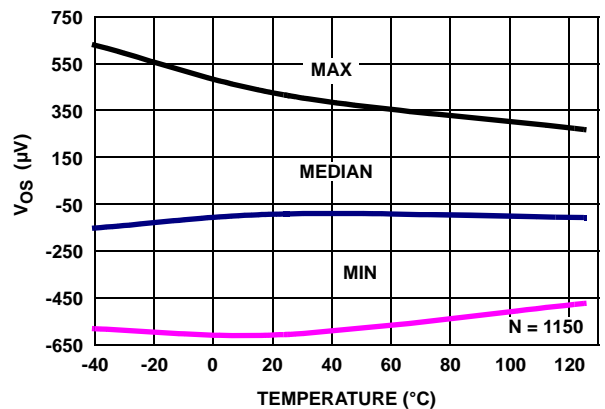
FIGURE 23. V_{OS} (SOT PKG) vs TEMPERATURE, V_+ = 5V , V_- = \pm 1.2V
