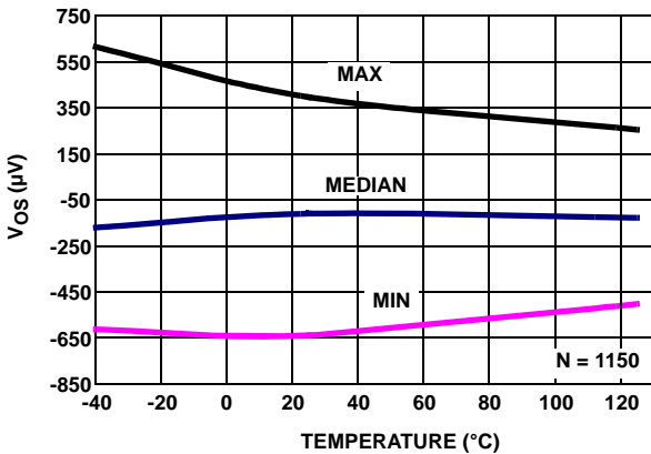
FIGURE 22. V_{OS} (SOT PKG) vs TEMPERATURE, V_+ = 5V , V_- = \pm 2.5V
