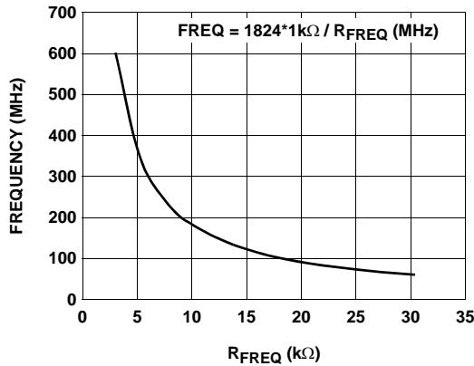
FIGURE 3. FREQUENCY vs R_{FREQ}
