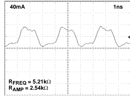
FIGURE 16. OUTPUT CURRENT @ 350MHz
