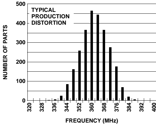
FIGURE 1. FREQUENCY DISTRIBUTION
