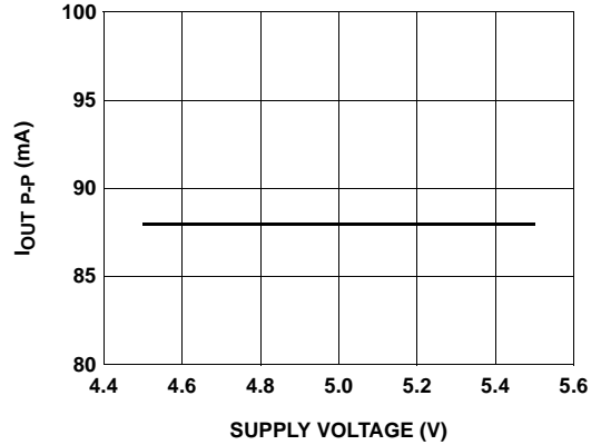
FIGURE 10. PEAK-TO-PEAK OUTPUT CURRENT vs SUPPLY VOLTAGE
