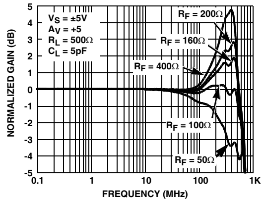
FIGURE 12. GAIN vs FREQUENCY FOR VARIOUS R_F ( A_V = +5 )
