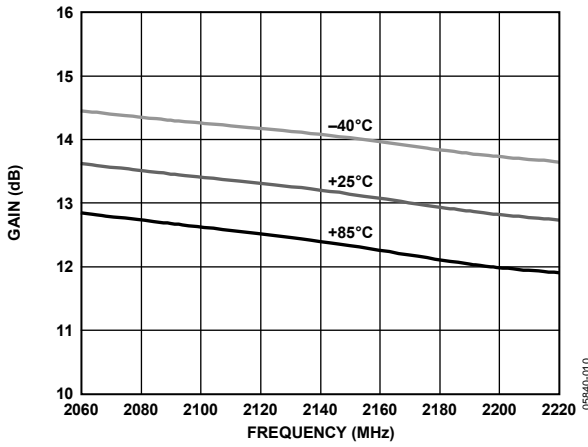
Figure 10. Gain vs. Frequency and Temperature, 2060 MHz to 2200 MHz
